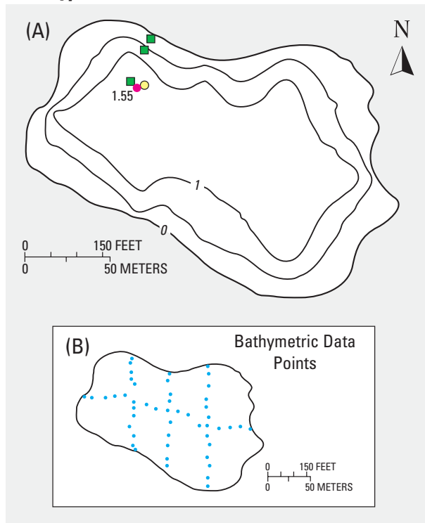
Figure 7. (A) Wetland bathymetric contours, (B) density of bathymetric data points, and (C) stage-volume and stage-area curves for S-68 Cypress.
