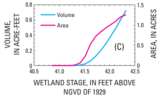
Figure 6. (A) Wetland bathymetric contours, (B) density of bathymetric data points, and (C) stage-volume and stage-area curves for S-63 Cypress.
