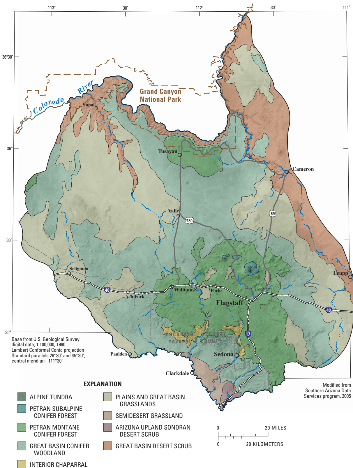
Figure 4. Vegetation types in the Coconino Plateau study area, Coconino and Yavapai Counties, Arizona.
