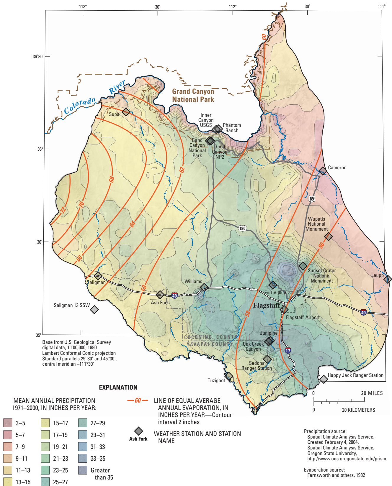
Figure 3. Mean and annual precipitation and average annual evaporation, Coconino Plateau study area, Coconino and Yavapai Counties, Arizona.
