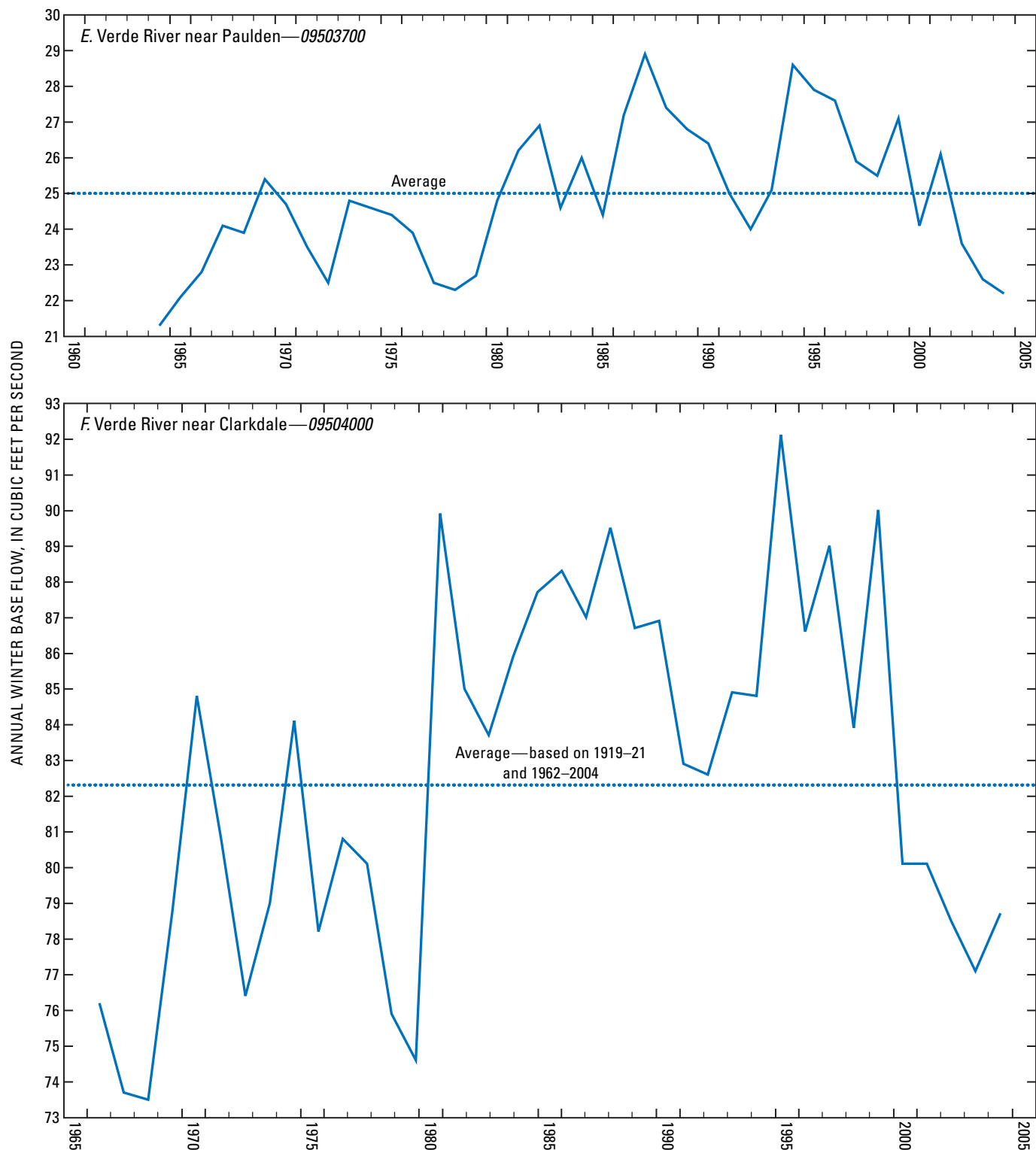
Figure 9. Annual winter base flow for selected streamflow-gaging stations, Coconino Plateau study area, Coconino and Yavapai Counties, Arizona: A , Havasu Creek below Havasu Springs at Supai; B , Havasu Creek above the mouth near Supai; C , Oak Creek near Sedona; D , Wet Beaver Creek near Rimrock; E , Verde River near Paulden; F , Verde River near Clarkdale—Continued.
