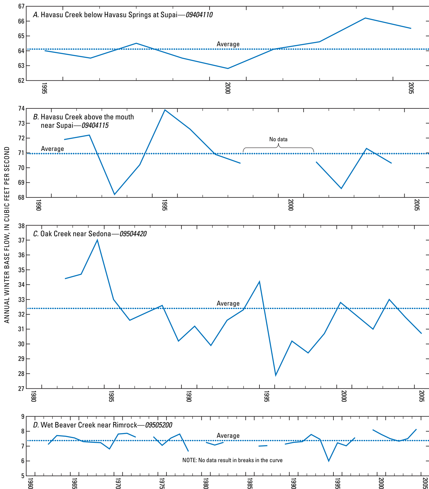
Figure 9. Annual winter base flow for selected streamflow-gaging stations, Coconino Plateau study area, Coconino and Yavapai Counties, Arizona: A, Havasu Creek below Havasu Springs at Supai; B, Havasu Creek above the mouth near Supai; C, Oak Creek near Sedona; D, Wet Beaver Creek near Rimrock; E, Verde River near Paulden; F, Verde River near Clarkdale.
