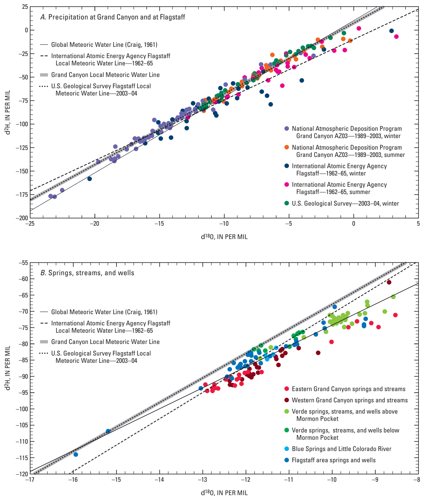
Figure 15. Oxygen and hydrogen data for precipitation and for springs, streams, and wells that are discharge points from the C aquifer and the Redwall-Muav aquifer, Coconino Plateau study area, Coconino and Yavapai Counties, Arizona: A , Precipitation at Grand Canyon 1989–2003, and at Flagstaff 1962–2004; B , Springs, streams, and wells, 1991–2004.
