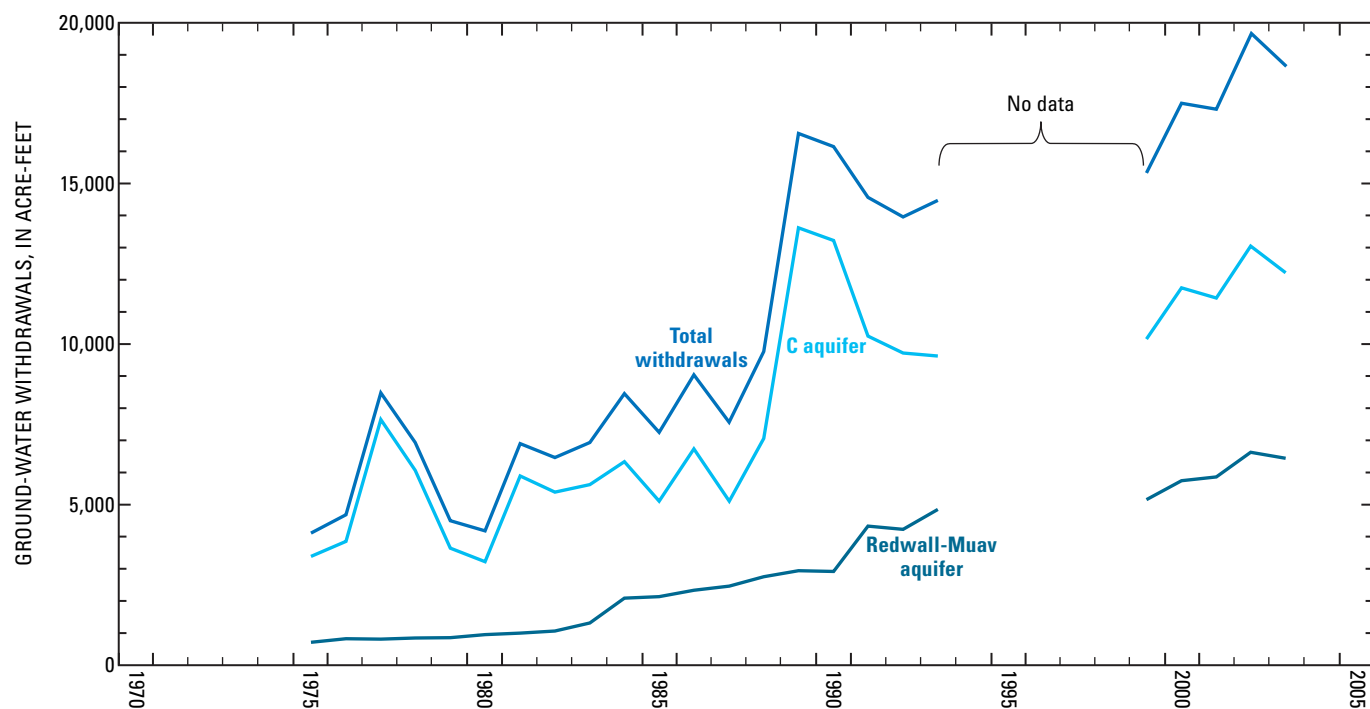
Figure 10. Annual and total ground-water withdrawals from the C aquifer and the Redwall-Muav aquifer in the Coconino Plateau study area, Arizona, 1975–2003.
