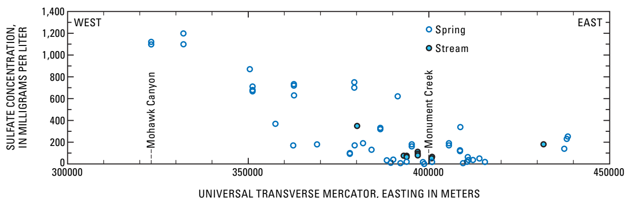
Figure 12. Concentrations of sulfate in relation to spring or stream locations near the south rim of Grand Canyon from the mouth of the Little Colorado River to Mohawk Canyon, Arizona, 1991–2002.
