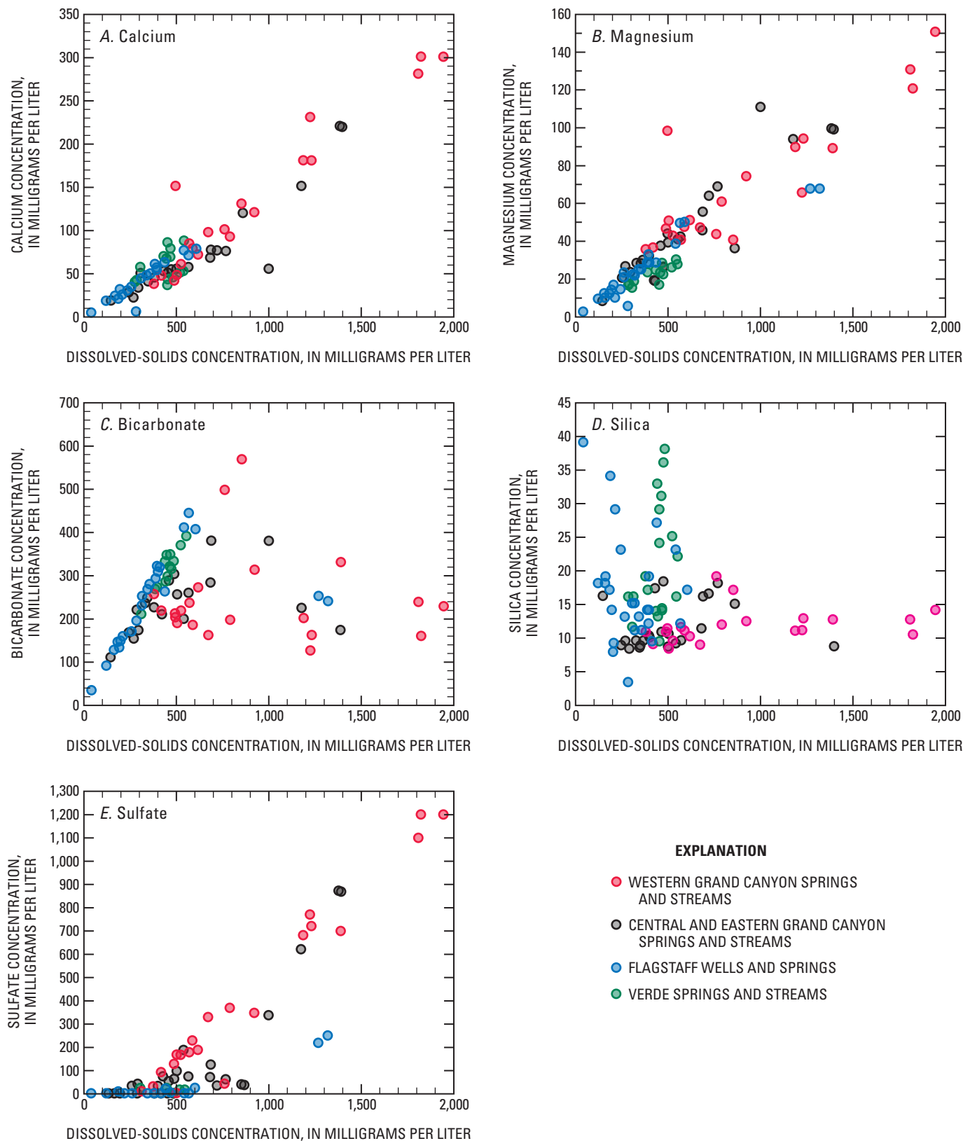
Figure 13. Relation between concentrations of dissolved solids and major ions in water from springs, streams, and wells in the Coconino Plateau study area, Coconino and Yavapai Counties, Arizona, 1921–2003: A , Calcium; B , Magnesium; C , Bicarbonate; D , Silica; and E , Sulfate.
