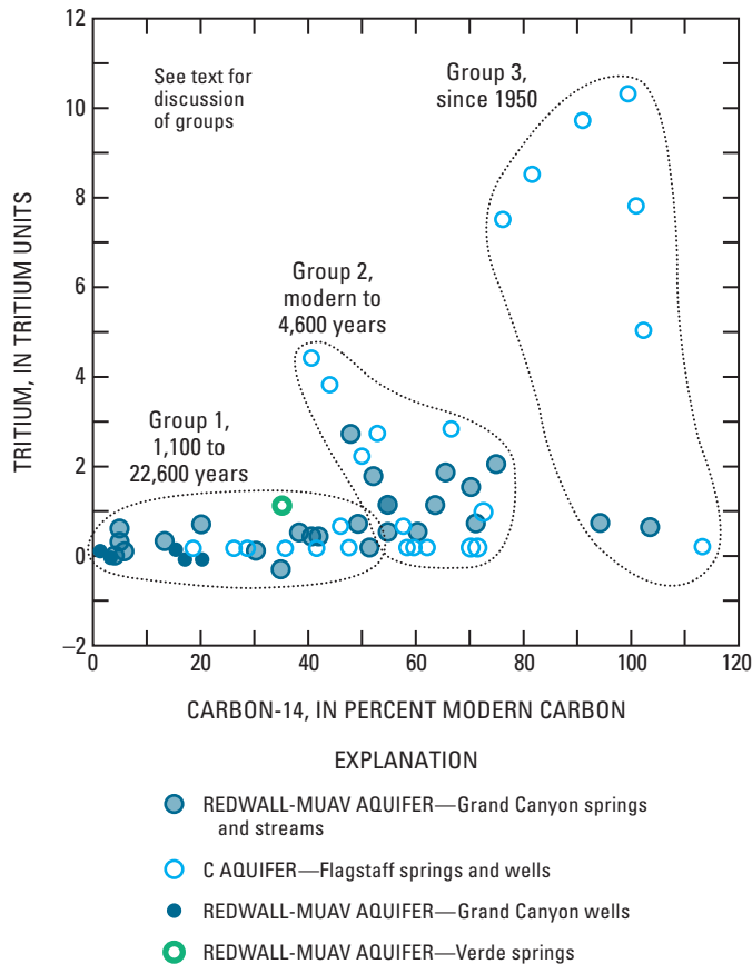
Figure 17. Relation between tritium and carbon-14 in water from springs, streams, and wells that are discharge points for the C aquifer and the Redwall-Muav aquifer, Coconino Plateau study area, Coconino and Yavapai Counties, Arizona, 1991–2003.
