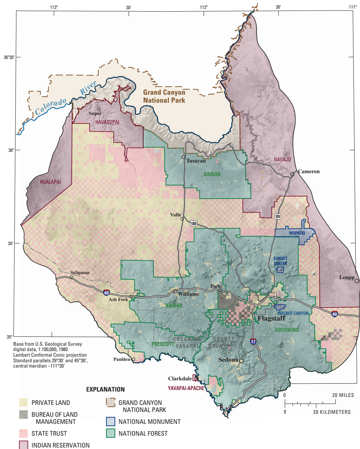
Figure 5. Land ownership in the Coconino Plateau study area, Coconino and Yavapai Counties, Arizona (modified from Southern Arizona Data Services Program, 2005).
