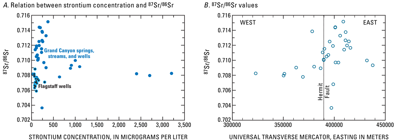
Figure 16. Strontium isotope values for water, Coconino Plateau study area, Coconino and Yavapai Counties, Arizona 2000–2003: A, Relation between strontium concentrations and ^{87}\text{Sr}/^{86}\text{Sr} in water from wells near Flagstaff and springs, streams, and wells near Grand Canyon; B, ^{87}\text{Sr}/^{86}\text{Sr} values in relation to spring or stream locations near the south rim of Grand Canyon.
