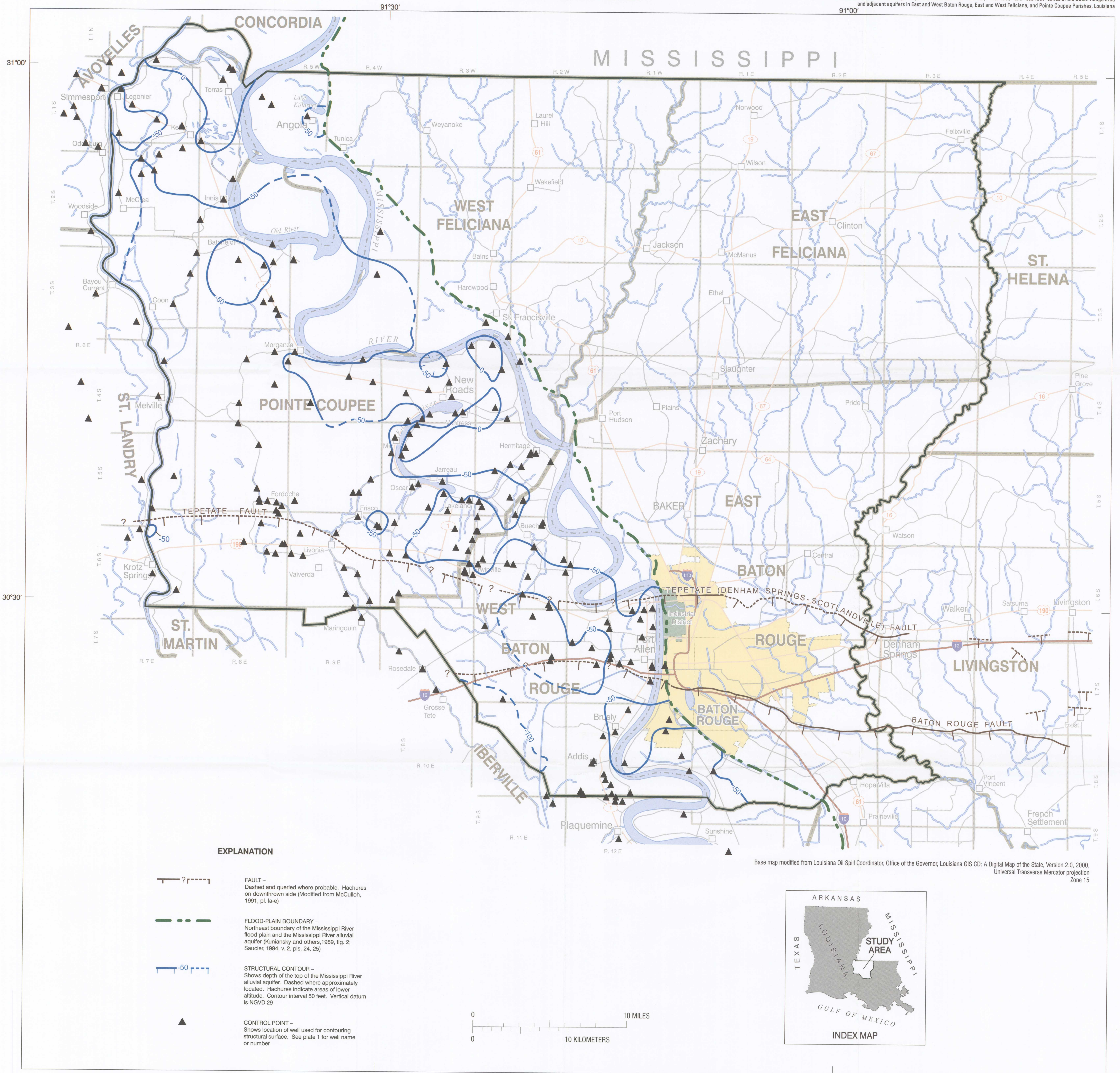
Plate 2. Altitude of the top of the Mississippi River alluvial aquifer in East and West Baton Rouge, East and West Feliciana, and Pointe Coupee Parishes, southeastern Louisiana.
