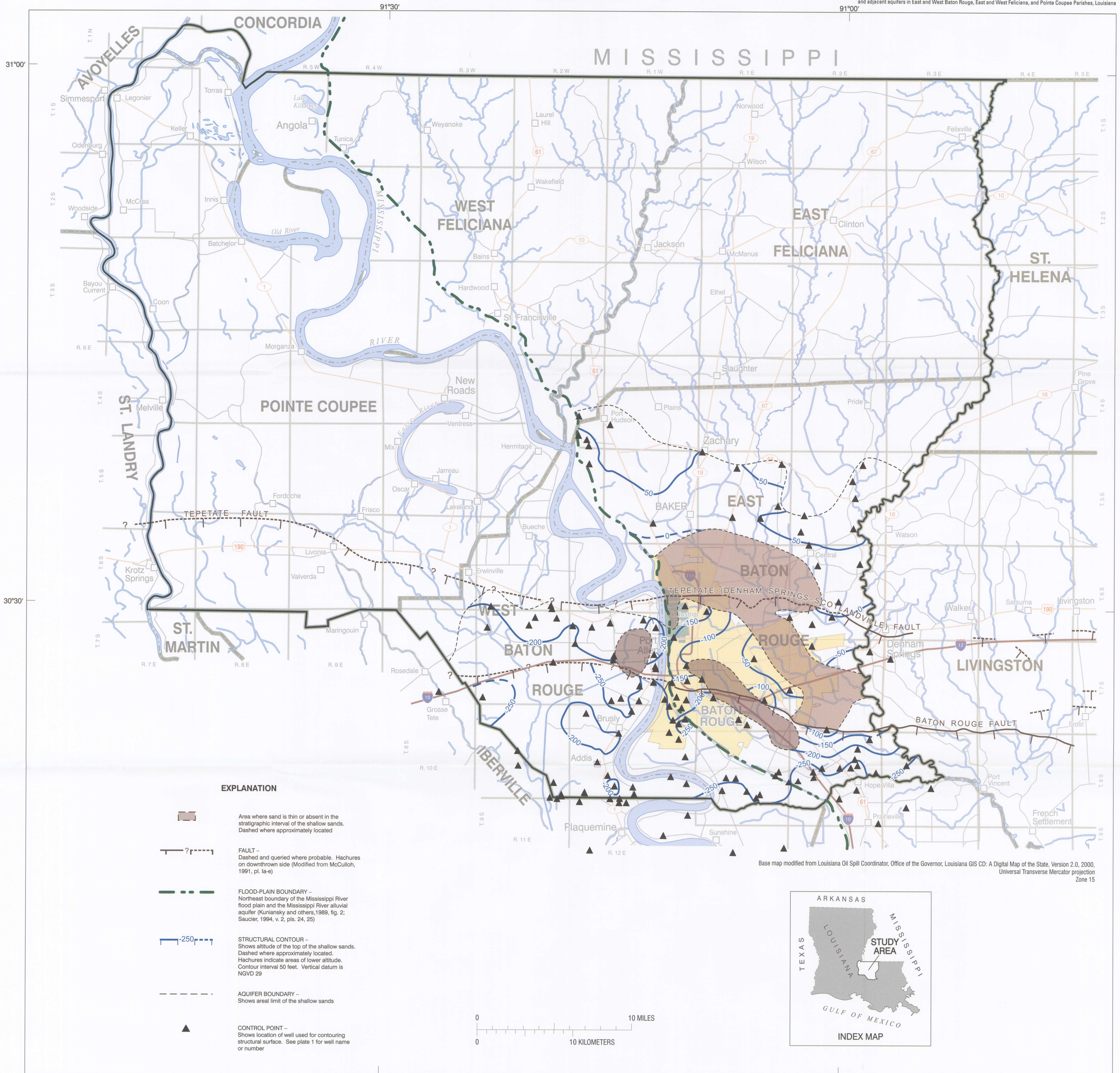
Plate 4. Altitude of the top of the shallow sands of the Baton Rouge area in East and West Baton Rouge, East and West Feliciana, and Pointe Coupee Parishes, southeastern Louisiana.
