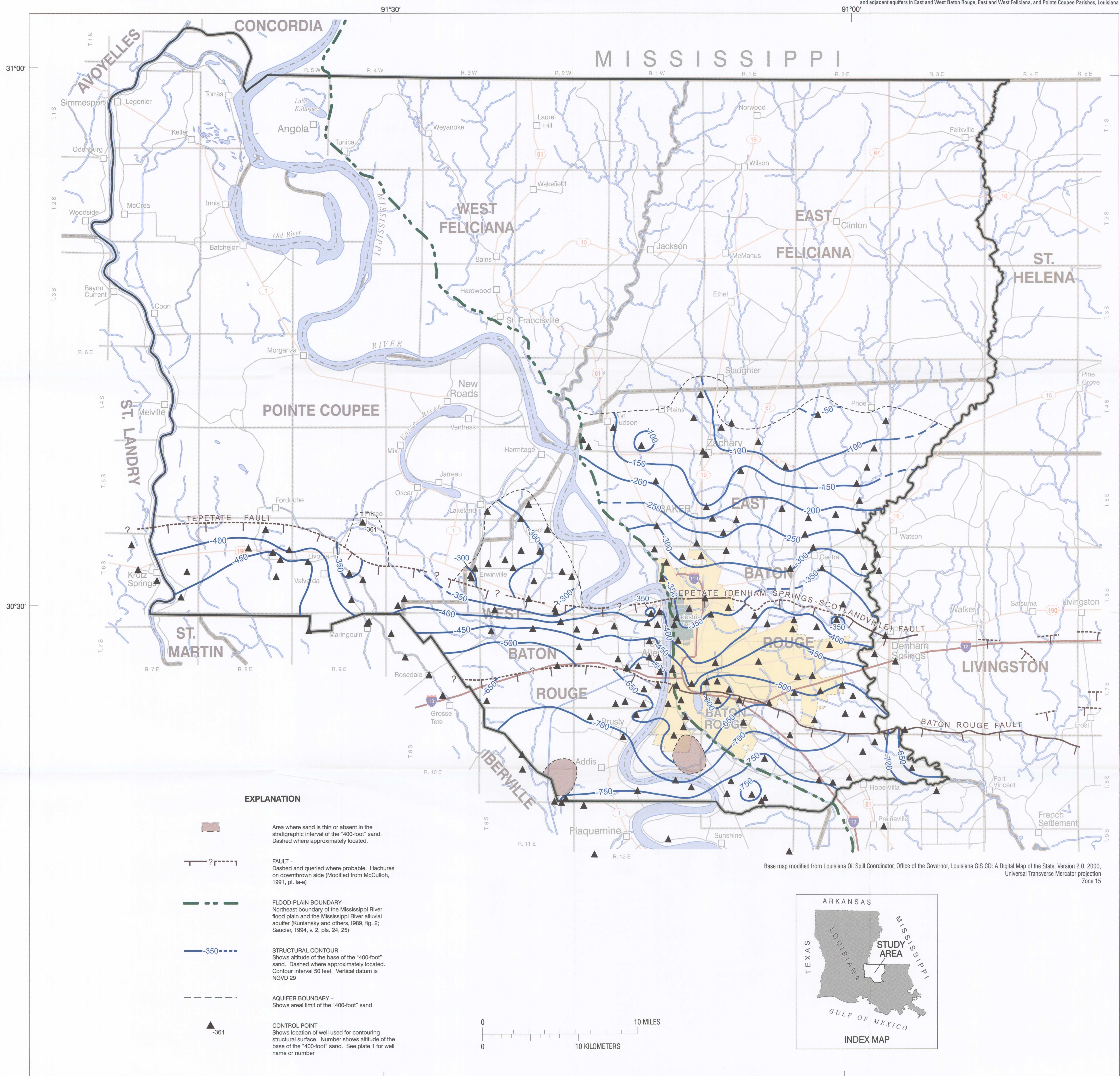
Plate 9. Altitude of the base of the "400-foot" sand of the Baton Rouge area in East and West Baton Rouge, East and West Feliciana, and Pointe Coupee Parishes, southeastern Louisiana.
