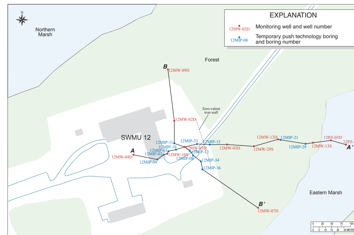
Trace of hydrogeologic section A-A' and B-B'
