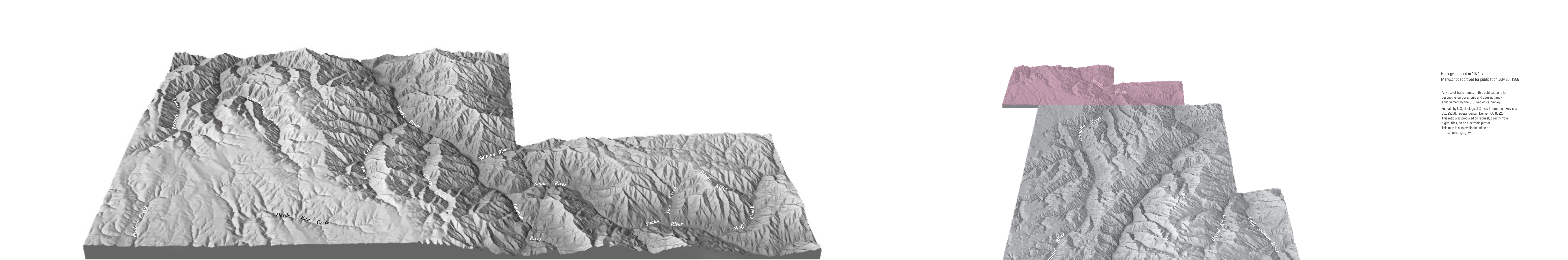
SHADED RELIEF MAP OF PLATE 2 (NORTH PART) (Shaded relief derived from U.S. Geological Survey 10-meter DEMs) SHADED RELIEF MAP OF PLATES 1 and 2 Shaded relief derived from U.S. Geological Survey 10-meter DEMs. Color indicates area mapped on this part of plate.
