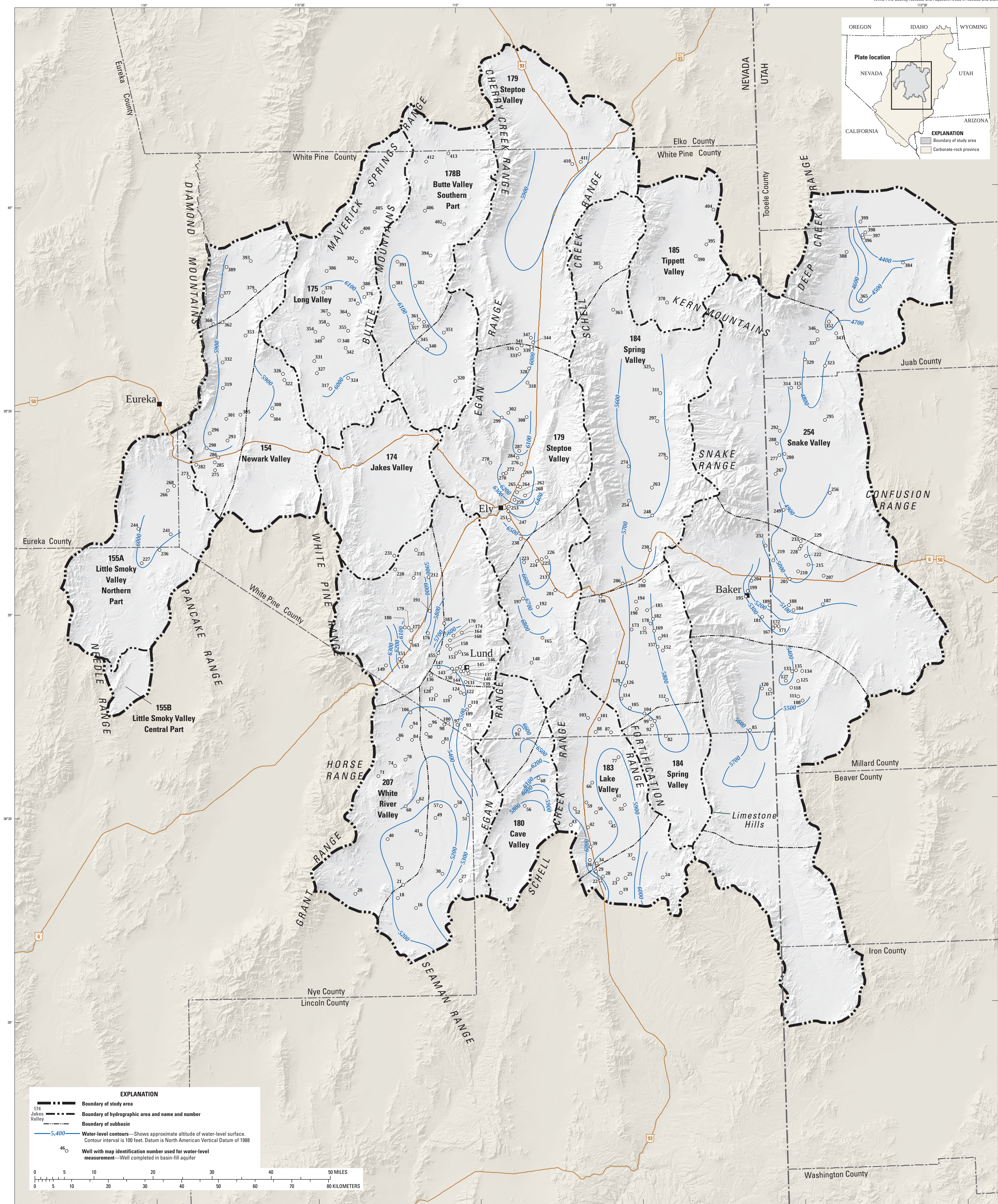
ALTITUDE OF WATER TABLE IN THE BASIN-FILL AQUIFER, WHITE PINE COUNTY, NEVADA, AND ADJACENT AREAS IN NEVADA AND UTAH
