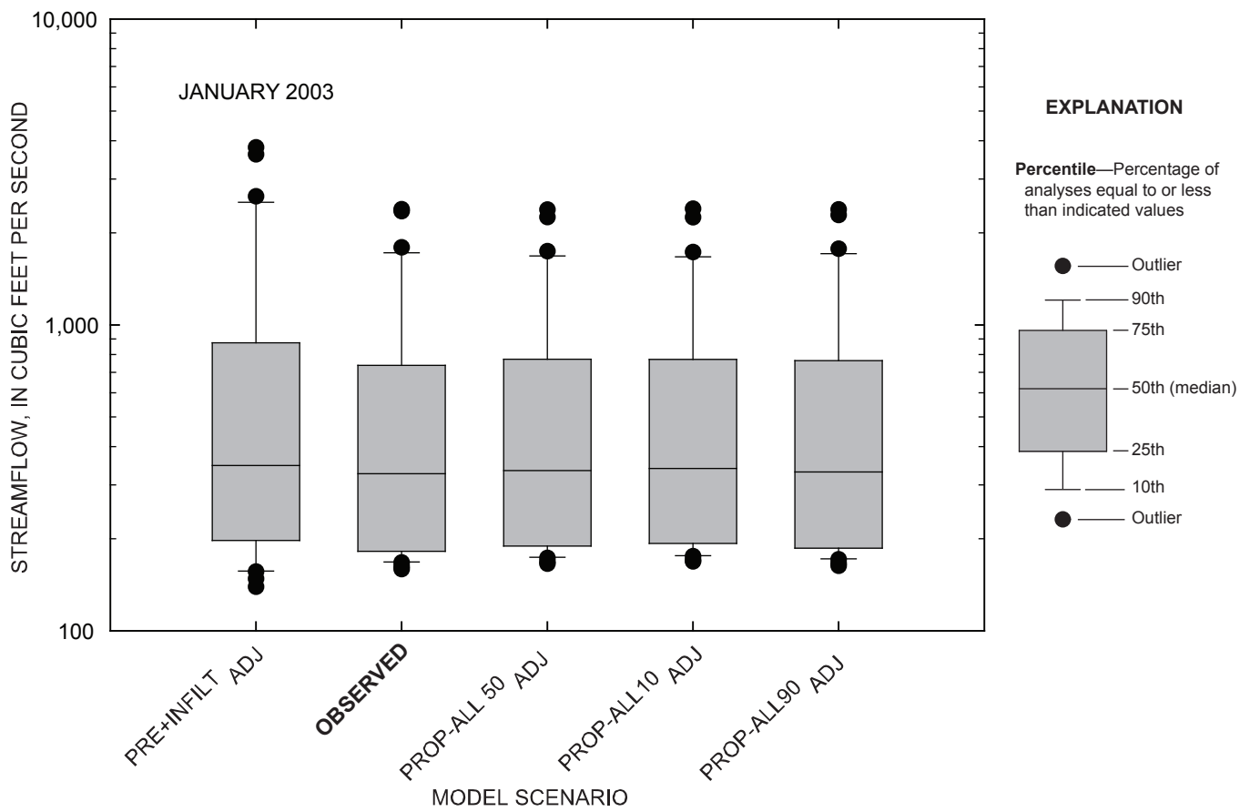
Figure 4-100. Comparison of daily streamflow for observed and simulated conditions at the Marais des Cygnes River near the Kansas-Missouri state line, Kansas, January 2003.
