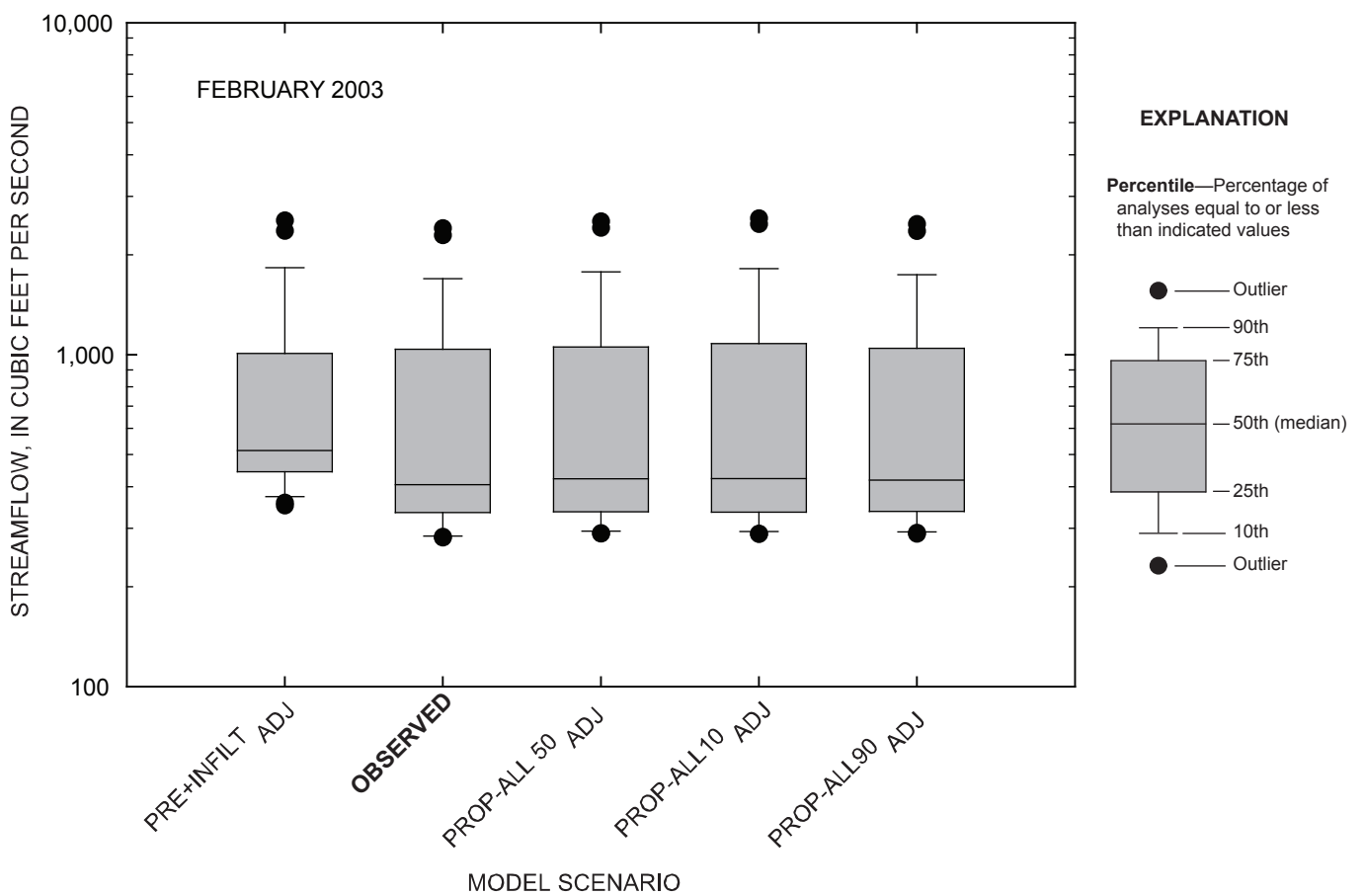
Figure 4-101. Comparison of daily streamflow for observed and simulated conditions at the Marais des Cygnes River near the Kansas-Missouri state line, Kansas, February 2003.
