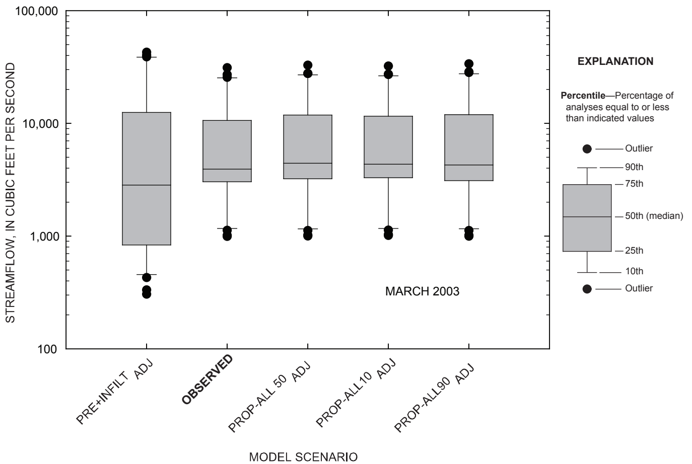
Figure 4-102. Comparison of daily streamflow for observed and simulated conditions at the Marais des Cygnes River near the Kansas-Missouri state line, Kansas, March 2003.
