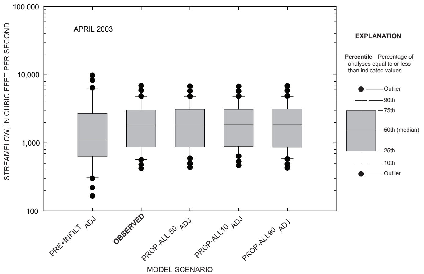
Figure 4-103. Comparison of daily streamflow for observed and simulated conditions at the Marais des Cygnes River near the Kansas-Missouri state line, Kansas, April 2003.
