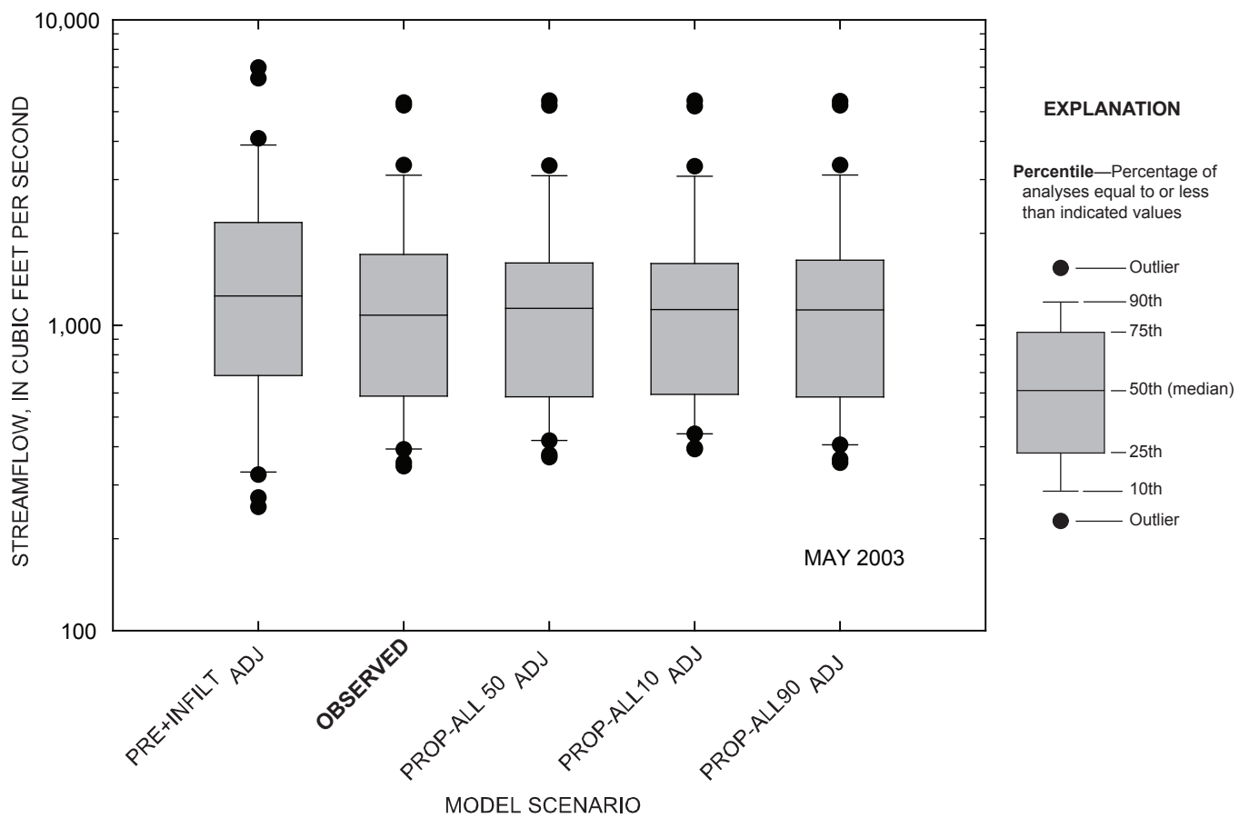
Figure 4-104. Comparison of daily streamflow for observed and simulated conditions at the Marais des Cygnes River near the Kansas-Missouri state line, Kansas, May 2003.
