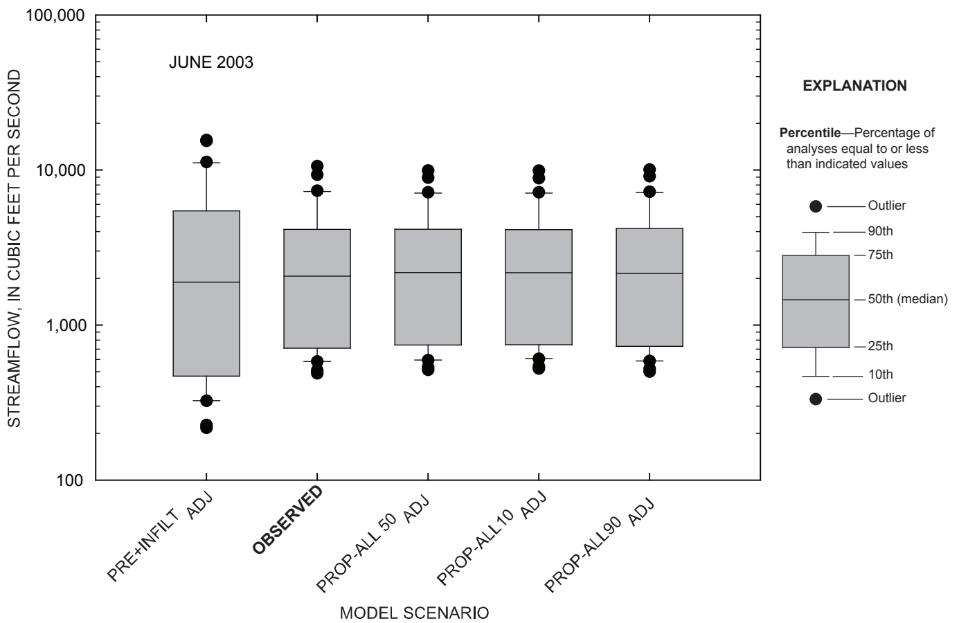
Figure 4-105. Comparison of daily streamflow for observed and simulated conditions at the Marais des Cygnes River near the Kansas-Missouri state line, Kansas, June 2003.
