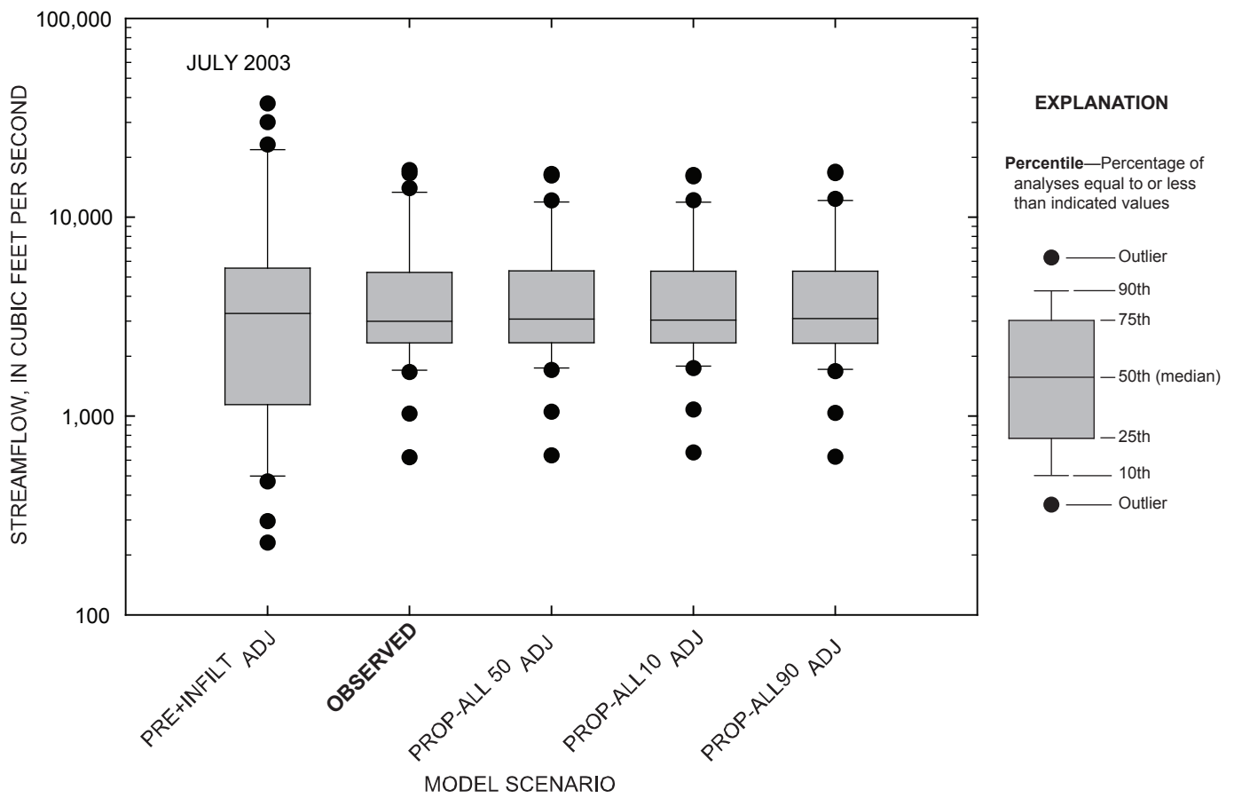
Figure 4-106. Comparison of daily streamflow for observed and simulated conditions at the Marais des Cygnes River near the Kansas-Missouri state line, Kansas, July 2003.
