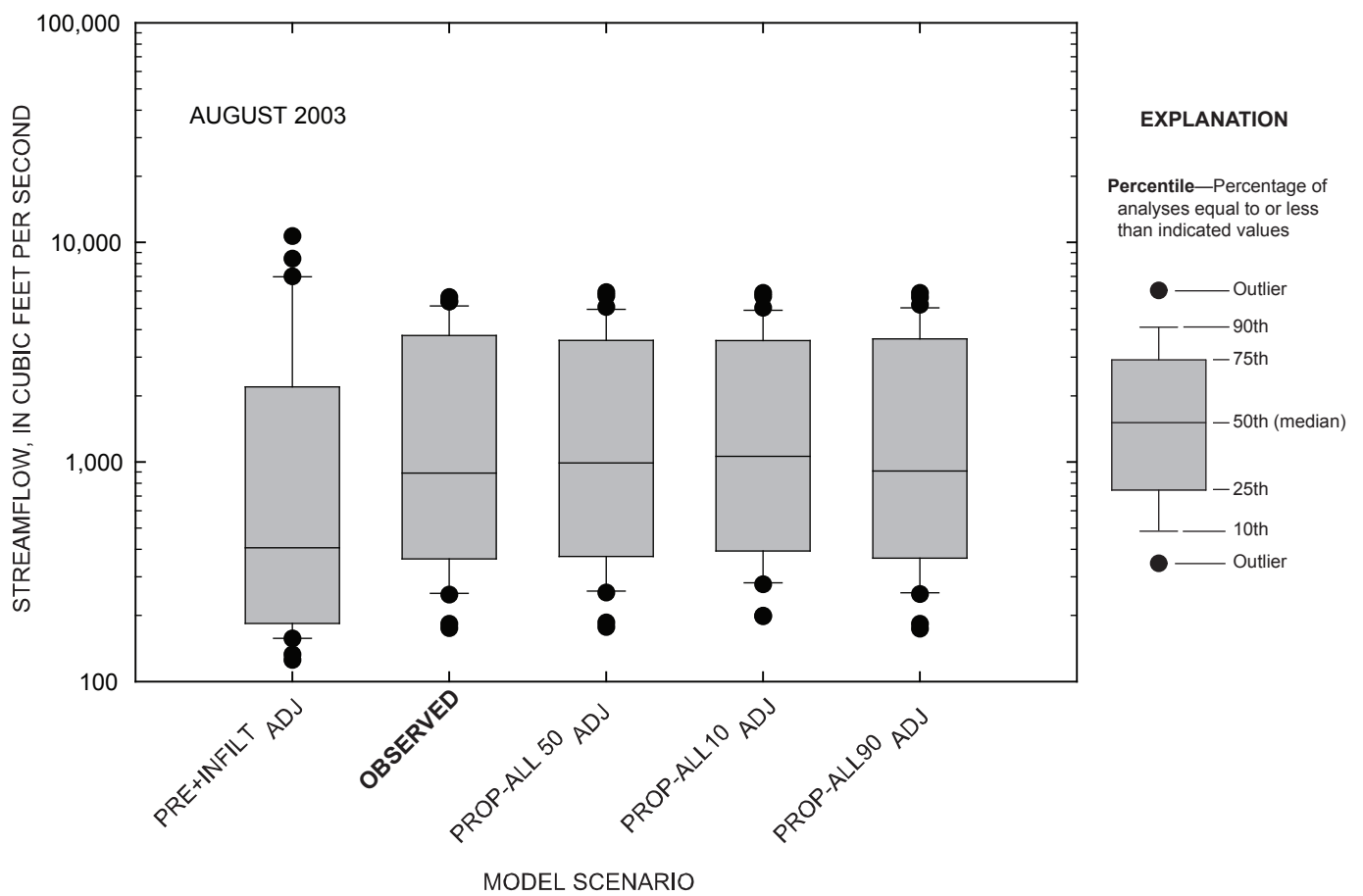
Figure 4-107. Comparison of daily streamflow for observed and simulated conditions at the Marais des Cygnes River near the Kansas-Missouri state line, Kansas, August 2003.
