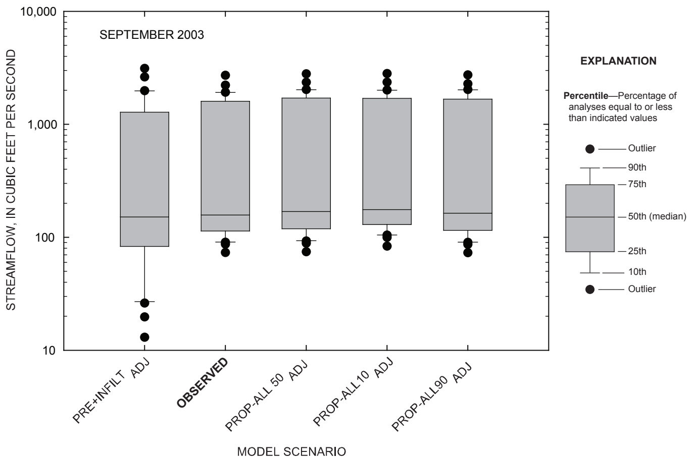
Figure 4-108. Comparison of daily streamflow for observed and simulated conditions at the Marais des Cygnes River near the Kansas-Missouri state line, Kansas, September 2003.
