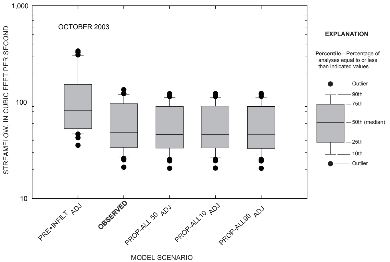
Figure 4-109. Comparison of daily streamflow for observed and simulated conditions at the Marais des Cygnes River near the Kansas-Missouri state line, Kansas, October 2003.
