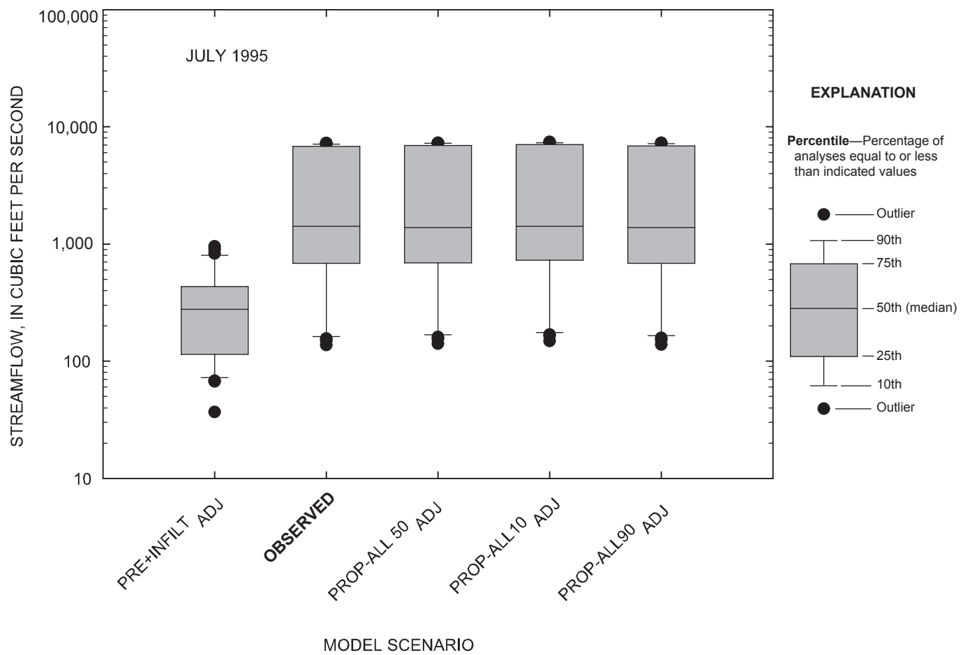
Figure 4-10. Comparison of daily streamflow for observed and simulated conditions at the Marais des Cygnes River near the Kansas-Missouri state line, Kansas, July 1995.
