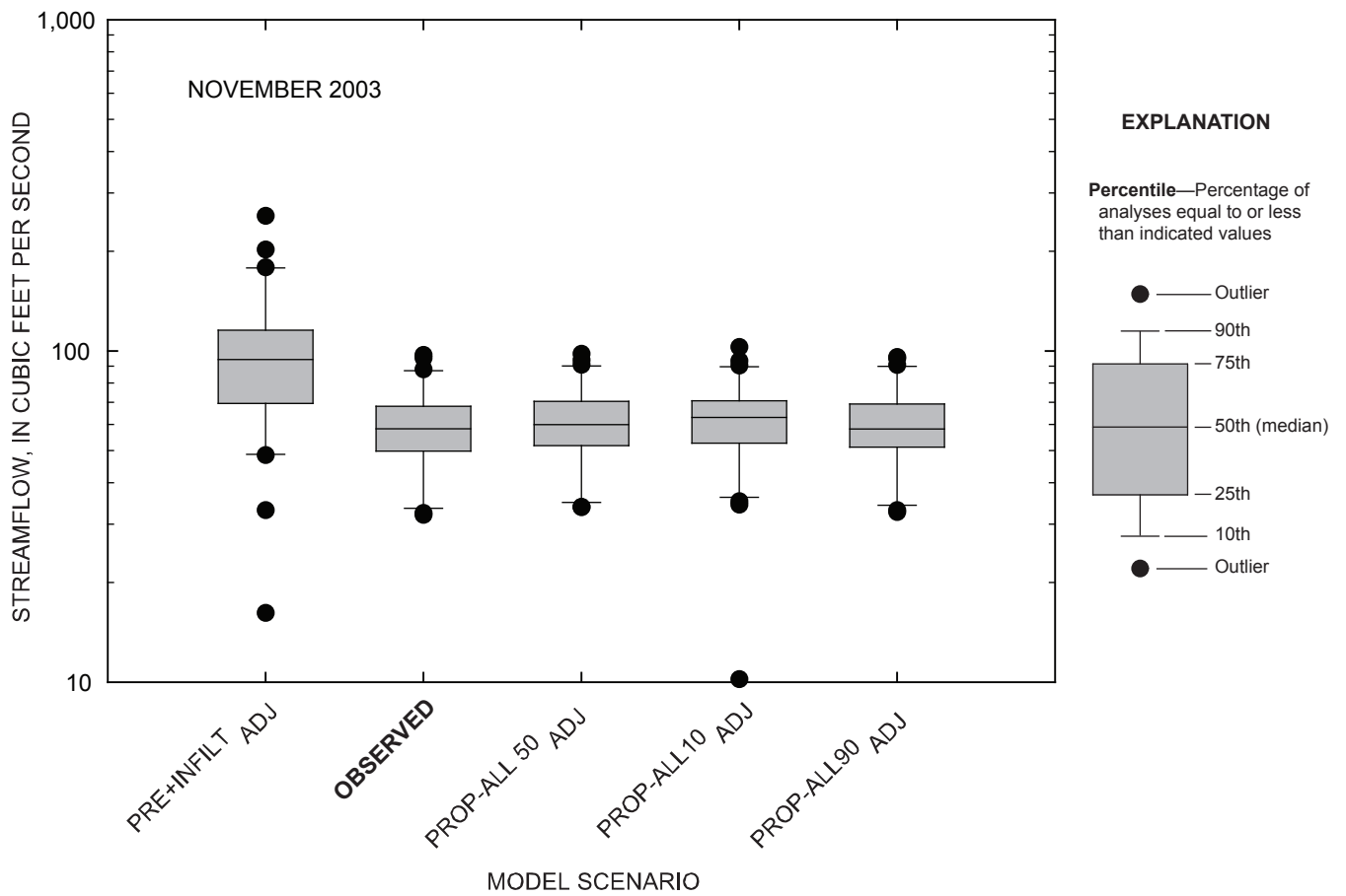
Figure 4-110. Comparison of daily streamflow for observed and simulated conditions at the Marais des Cygnes River near the Kansas-Missouri state line, Kansas, November 2003.
