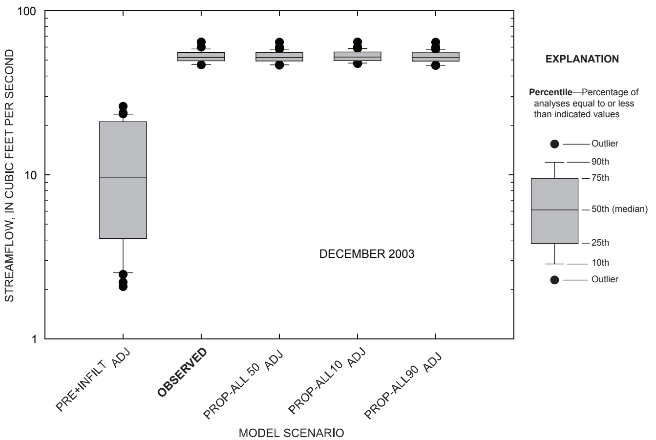
Figure 4-111. Comparison of daily streamflow for observed and simulated conditions at the Marais des Cygnes River near the Kansas-Missouri state line, Kansas, December 2003.
