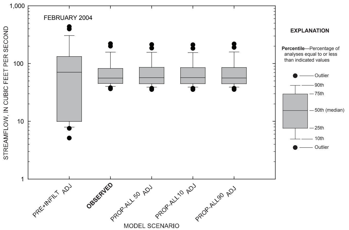
Figure 4-113. Comparison of daily streamflow for observed and simulated conditions at the Marais des Cygnes River near the Kansas-Missouri state line, Kansas, February 2004.
