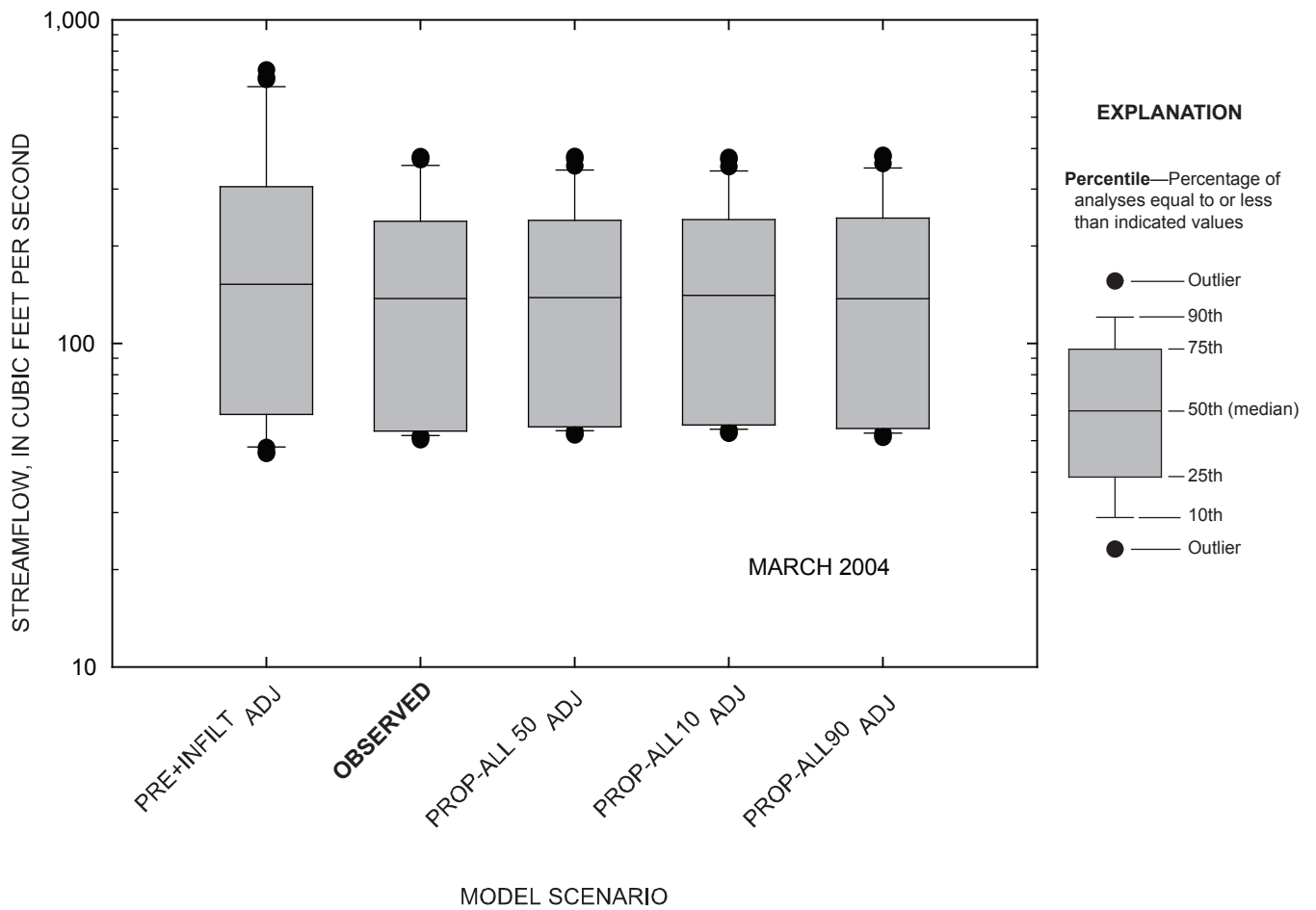
Figure 4-114. Comparison of daily streamflow for observed and simulated conditions at the Marais des Cygnes River near the Kansas-Missouri state line, Kansas, March 2004.
