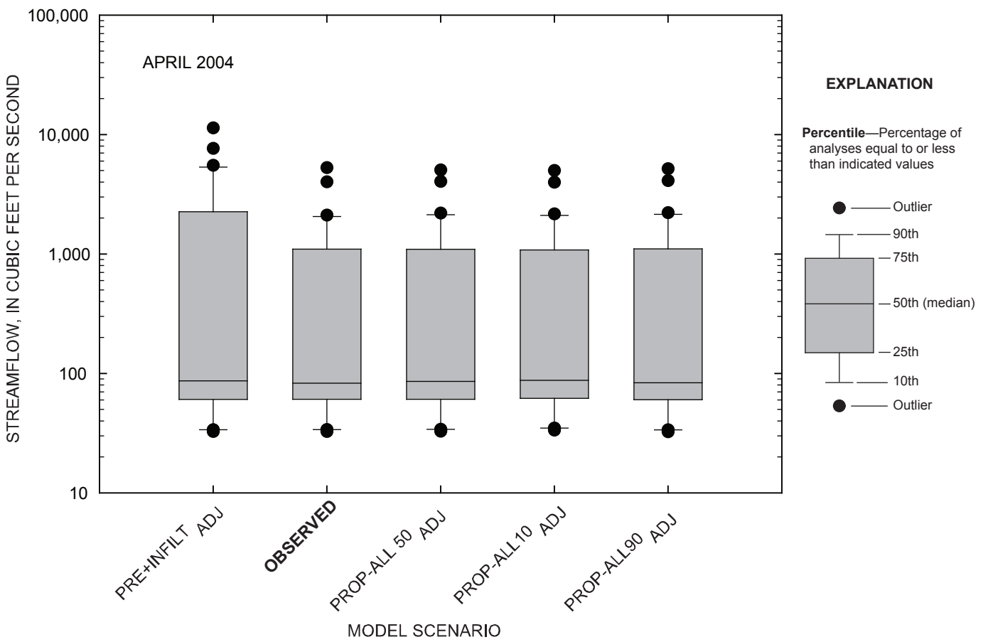
Figure 4-115. Comparison of daily streamflow for observed and simulated conditions at the Marais des Cygnes River near the Kansas-Missouri state line, Kansas, April 2004.
