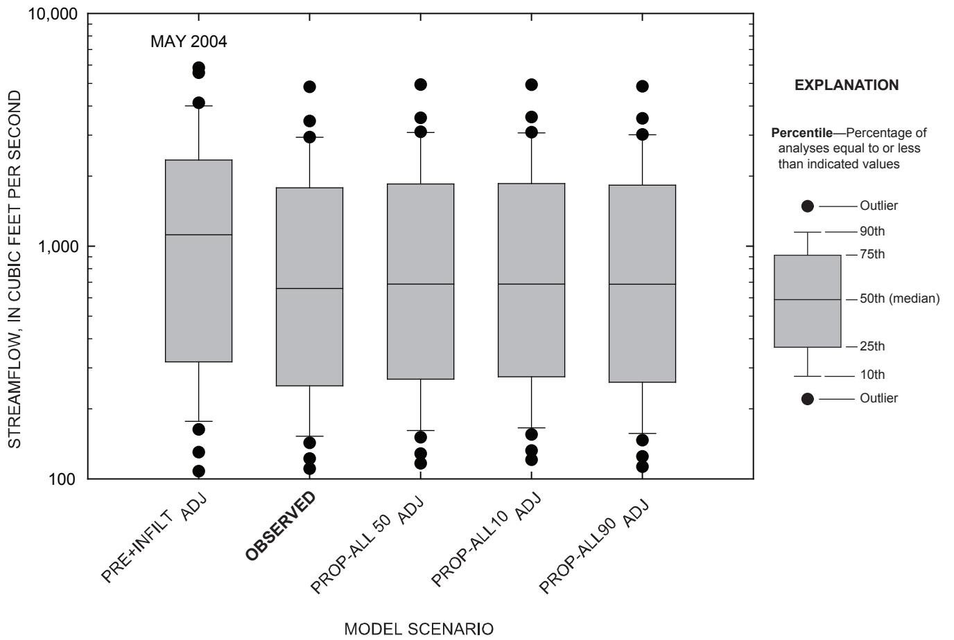
Figure 4-116. Comparison of daily streamflow for observed and simulated conditions at the Marais des Cygnes River near the Kansas-Missouri state line, Kansas, May 2004.
