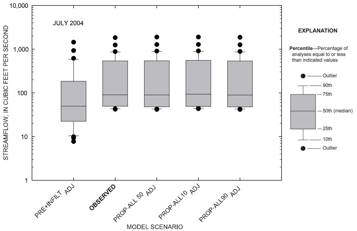
Figure 4-118. Comparison of daily streamflow for observed and simulated conditions at the Marais des Cygnes River near the Kansas-Missouri state line, Kansas, July 2004.
