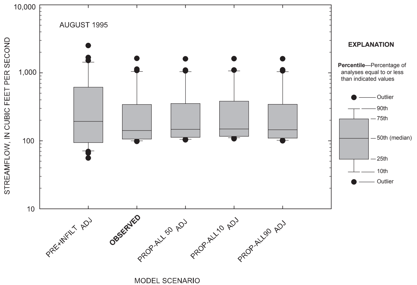
Figure 4-11. Comparison of daily streamflow for observed and simulated conditions at the Marais des Cygnes River near the Kansas-Missouri state line, Kansas, August 1995.
