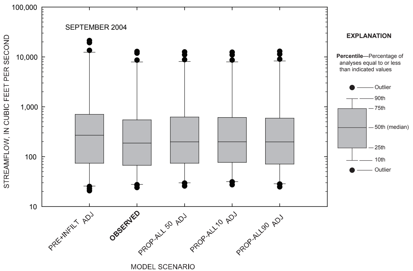
Figure 4-120. Comparison of daily streamflow for observed and simulated conditions at the Marais des Cygnes River near the Kansas-Missouri state line, Kansas, September 2004.
