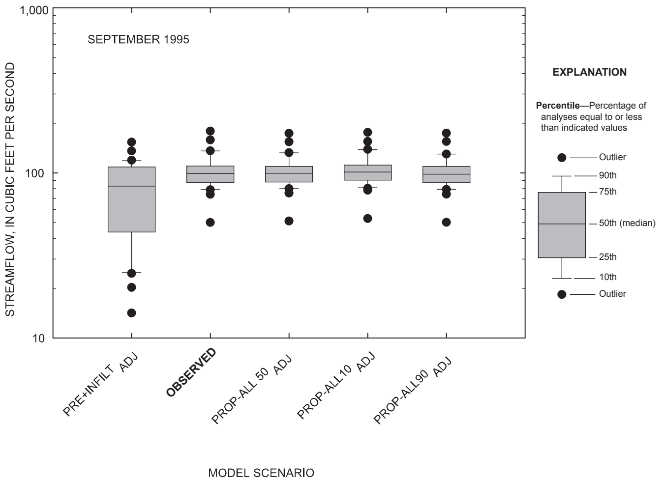
Figure 4-12. Comparison of daily streamflow for observed and simulated conditions at the Marais des Cygnes River near the Kansas-Missouri state line, Kansas, September 1995.
