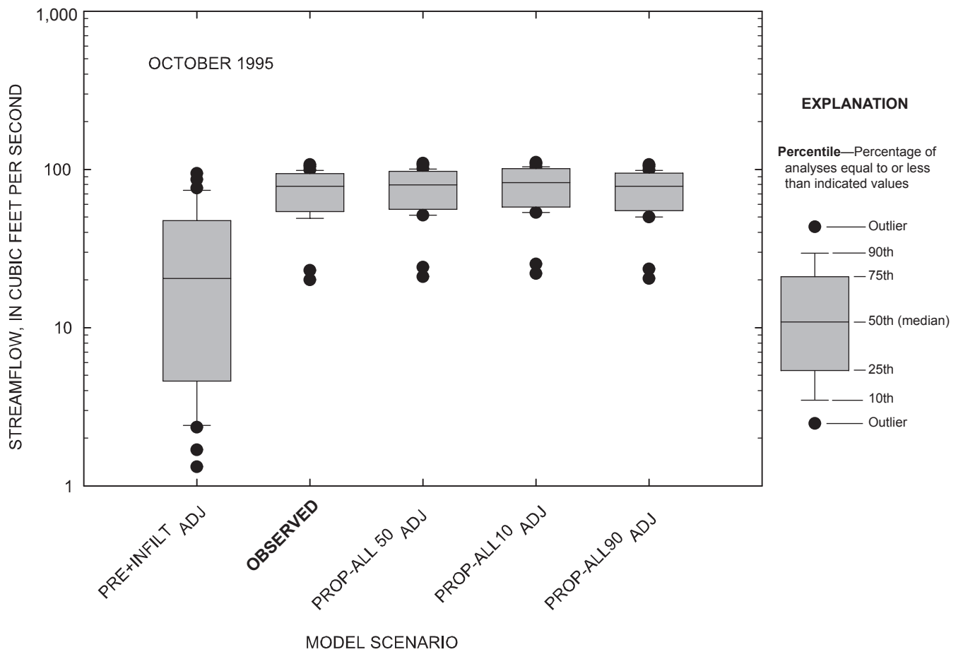
Figure 4-13. Comparison of daily streamflow for observed and simulated conditions at the Marais des Cygnes River near the Kansas-Missouri state line, Kansas, October 1995.
