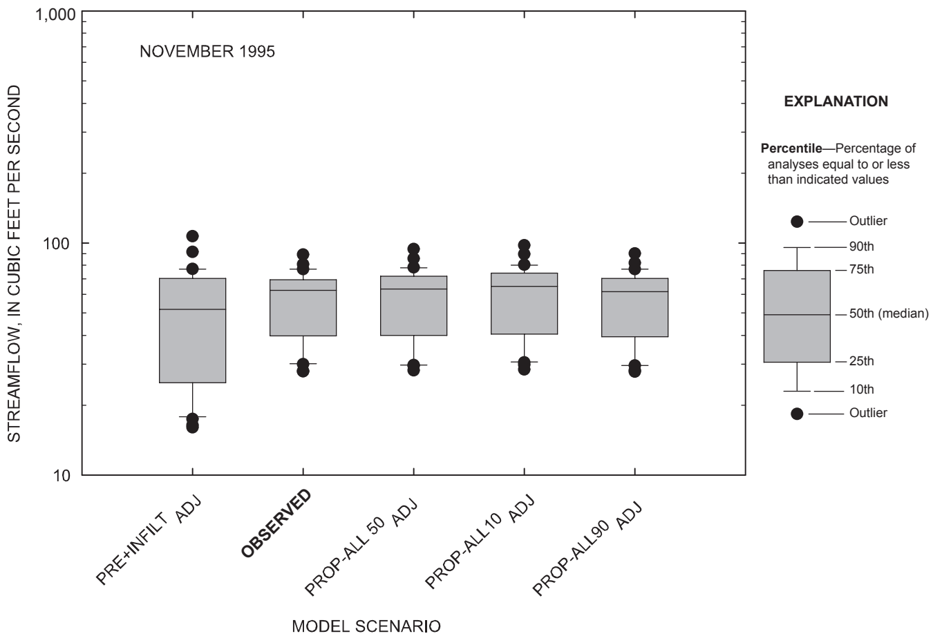
Figure 4-14. Comparison of daily streamflow for observed and simulated conditions at the Marais des Cygnes River near the Kansas-Missouri state line, Kansas, November 1995.
