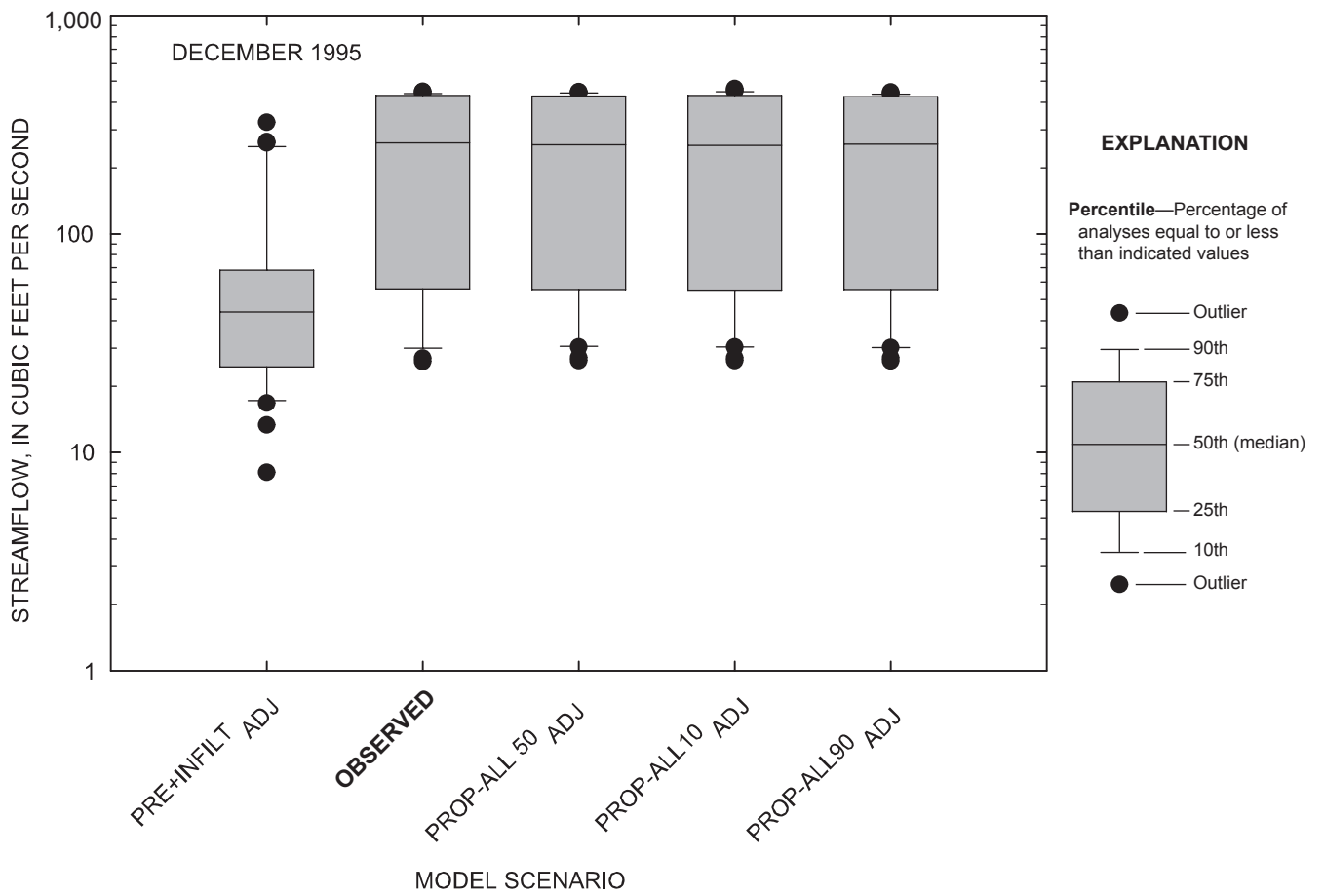
Figure 4-15. Comparison of daily streamflow for observed and simulated conditions at the Marais des Cygnes River near the Kansas-Missouri state line, Kansas, December 1995.
