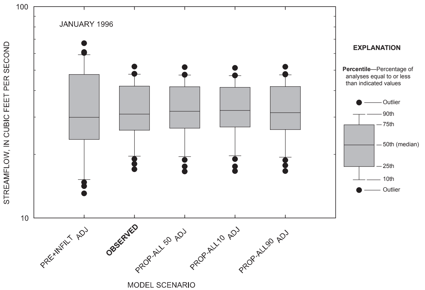
Figure 4-16. Comparison of daily streamflow for observed and simulated conditions at the Marais des Cygnes River near the Kansas-Missouri state line, Kansas, January 1996.
