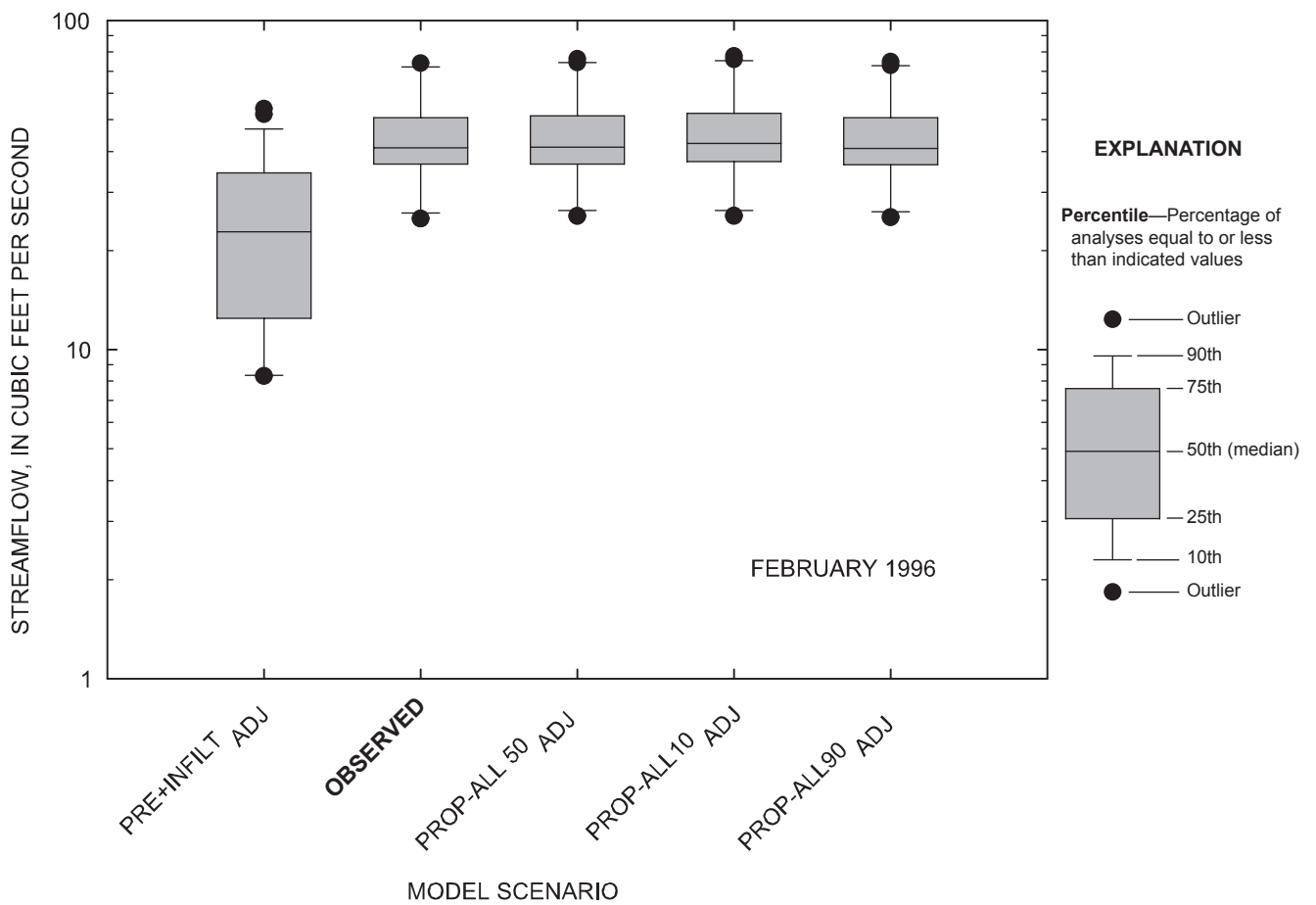
Figure 4-17. Comparison of daily streamflow for observed and simulated conditions at the Marais des Cygnes River near the Kansas-Missouri state line, Kansas, February 1996.
