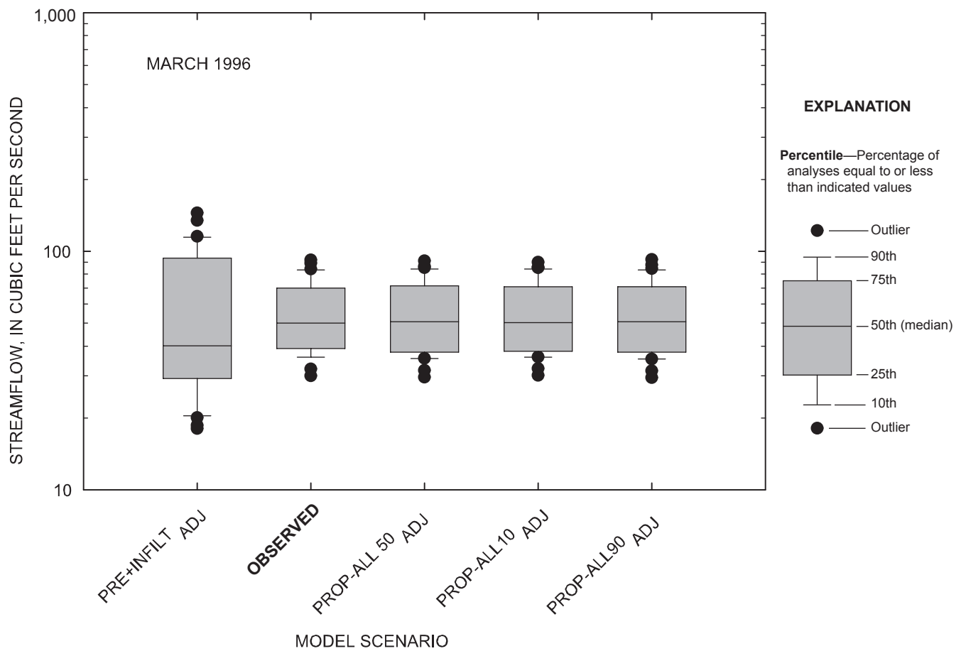
Figure 4-18. Comparison of daily streamflow for observed and simulated conditions at the Marais des Cygnes River near the Kansas-Missouri state line, Kansas, March 1996.
