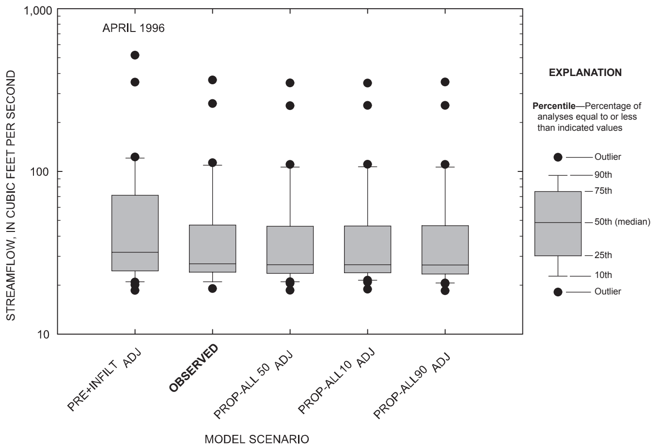
Figure 4-19. Comparison of daily streamflow for observed and simulated conditions at the Marais des Cygnes River near the Kansas-Missouri state line, Kansas, April 1996.
