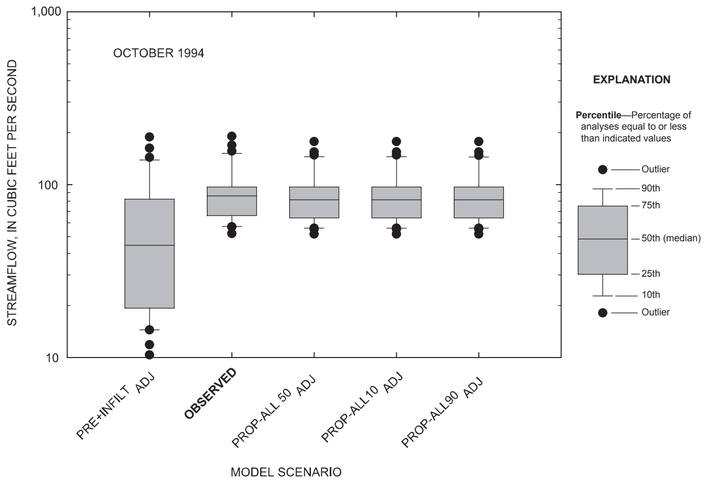
Figure 4-1. Comparison of daily streamflow for observed and simulated conditions at the Marais des Cygnes River near the Kansas-Missouri state line, Kansas, October 1994.
