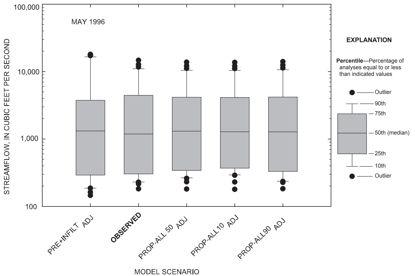
Figure 4-20. Comparison of daily streamflow for observed and simulated conditions at the Marais des Cygnes River near the Kansas-Missouri state line, Kansas, May 1996.
