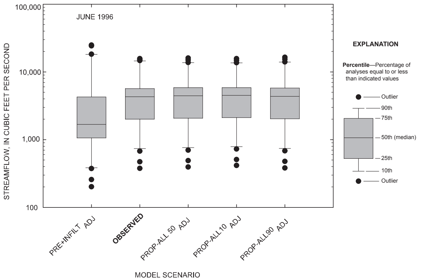
Figure 4-21. Comparison of daily streamflow for observed and simulated conditions at the Marais des Cygnes River near the Kansas-Missouri state line, Kansas, June 1996.
