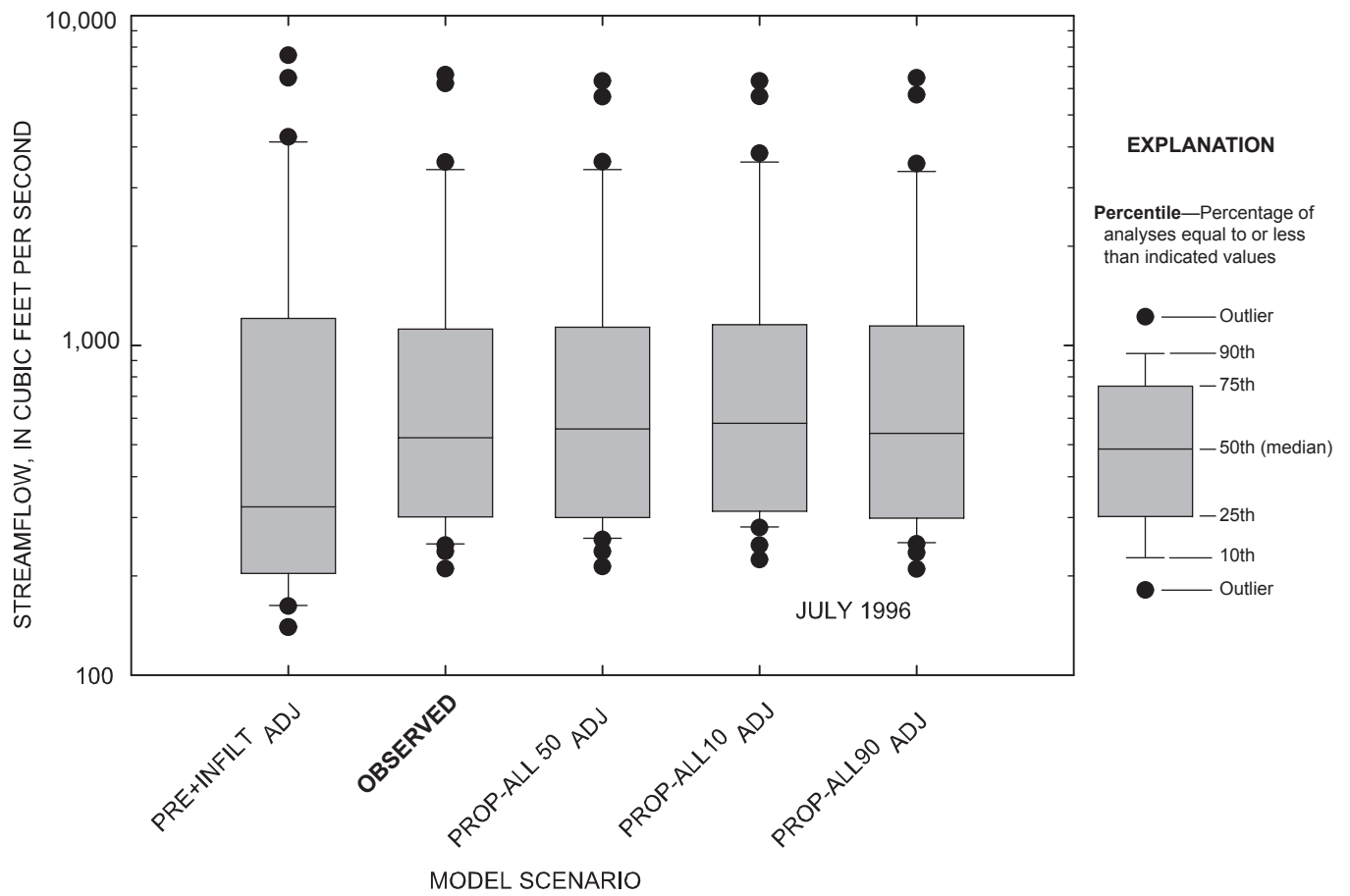
Figure 4-22. Comparison of daily streamflow for observed and simulated conditions at the Marais des Cygnes River near the Kansas-Missouri state line, Kansas, July 1996.
