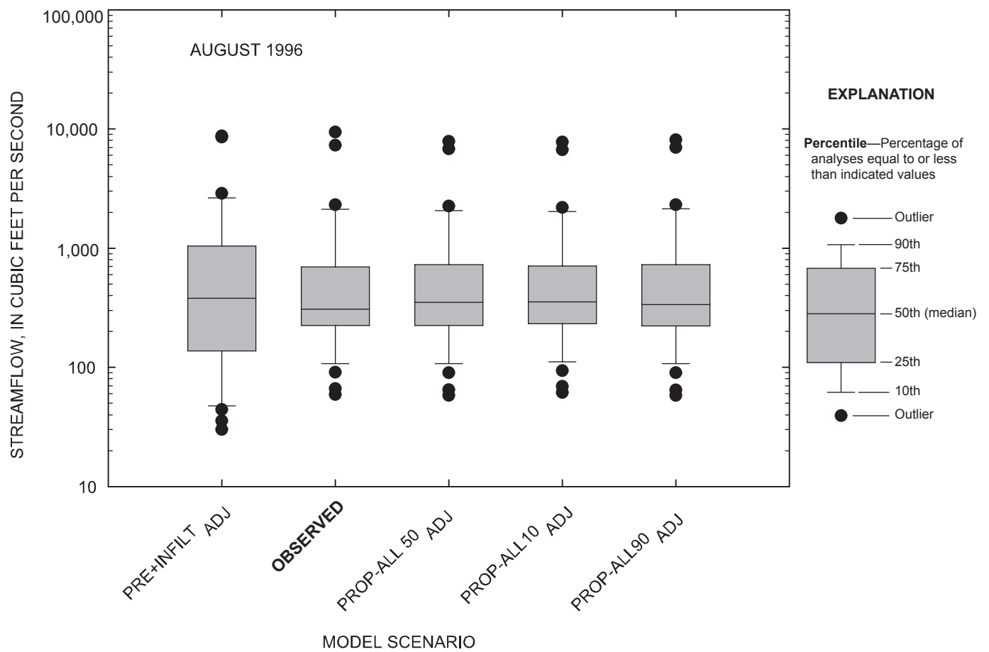
Figure 4-23. Comparison of daily streamflow for observed and simulated conditions at the Marais des Cygnes River near the Kansas-Missouri state line, Kansas, August 1996.
