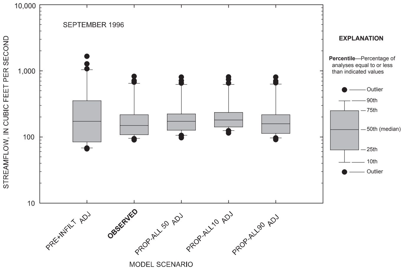
Figure 4-24. Comparison of daily streamflow for observed and simulated conditions at the Marais des Cygnes River near the Kansas-Missouri state line, Kansas, September 1996.
