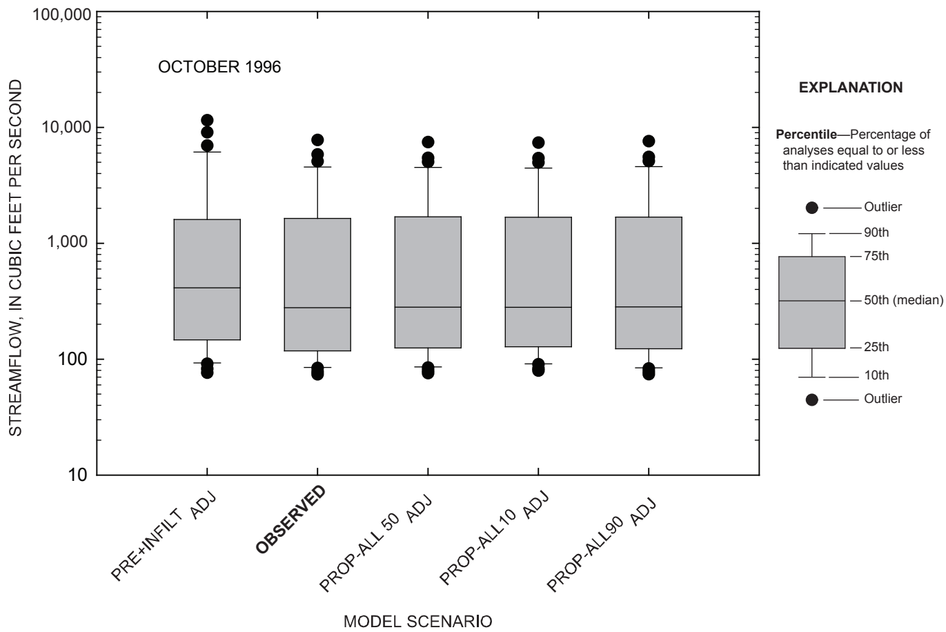
Figure 4-25. Comparison of daily streamflow for observed and simulated conditions at the Marais des Cygnes River near the Kansas-Missouri state line, Kansas, October 1996.
