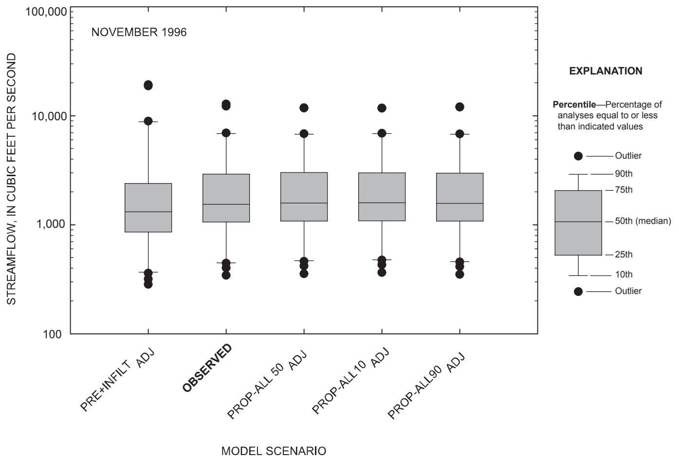
Figure 4-26. Comparison of daily streamflow for observed and simulated conditions at the Marais des Cygnes River near the Kansas-Missouri state line, Kansas, November 1996.
