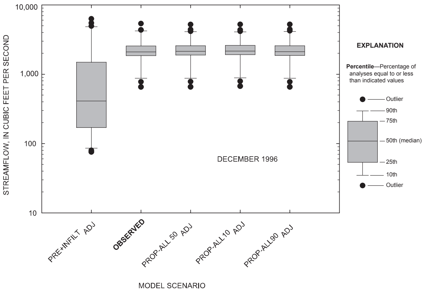
Figure 4-27. Comparison of daily streamflow for observed and simulated conditions at the Marais des Cygnes River near the Kansas-Missouri state line, Kansas, December 1996.
