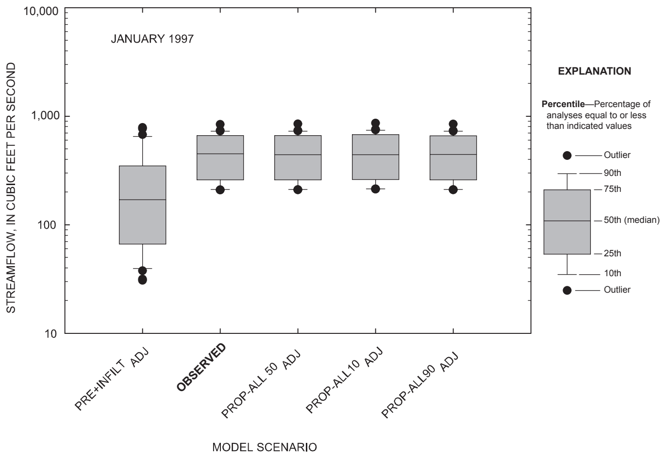
Figure 4-28. Comparison of daily streamflow for observed and simulated conditions at the Marais des Cygnes River near the Kansas-Missouri state line, Kansas, January 1997.
