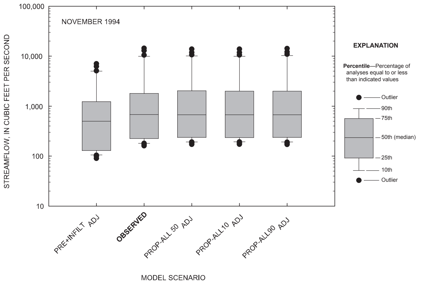
Figure 4-2. Comparison of daily streamflow for observed and simulated conditions at the Marais des Cygnes River near the Kansas-Missouri state line, Kansas, November 1994.
