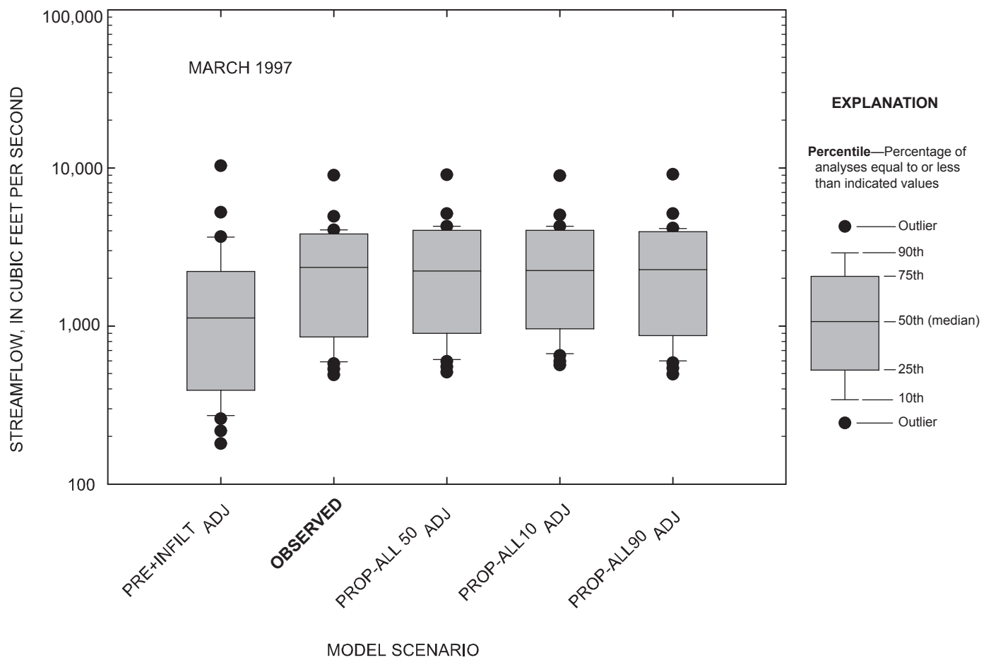
Figure 4-30. Comparison of daily streamflow for observed and simulated conditions at the Marais des Cygnes River near the Kansas-Missouri state line, Kansas, March 1997.
