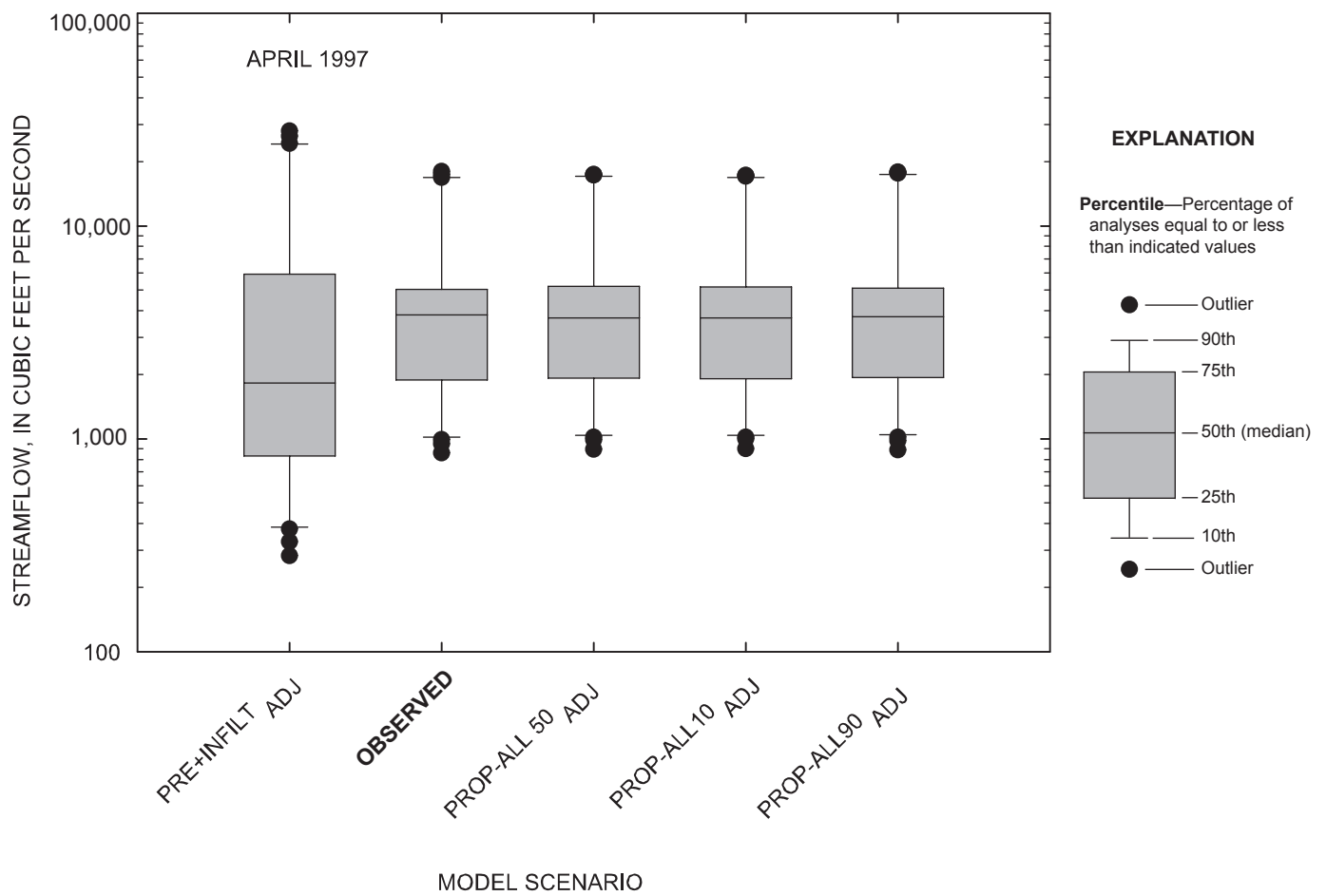
Figure 4-31. Comparison of daily streamflow for observed and simulated conditions at the Marais des Cygnes River near the Kansas-Missouri state line, Kansas, April 1997.
