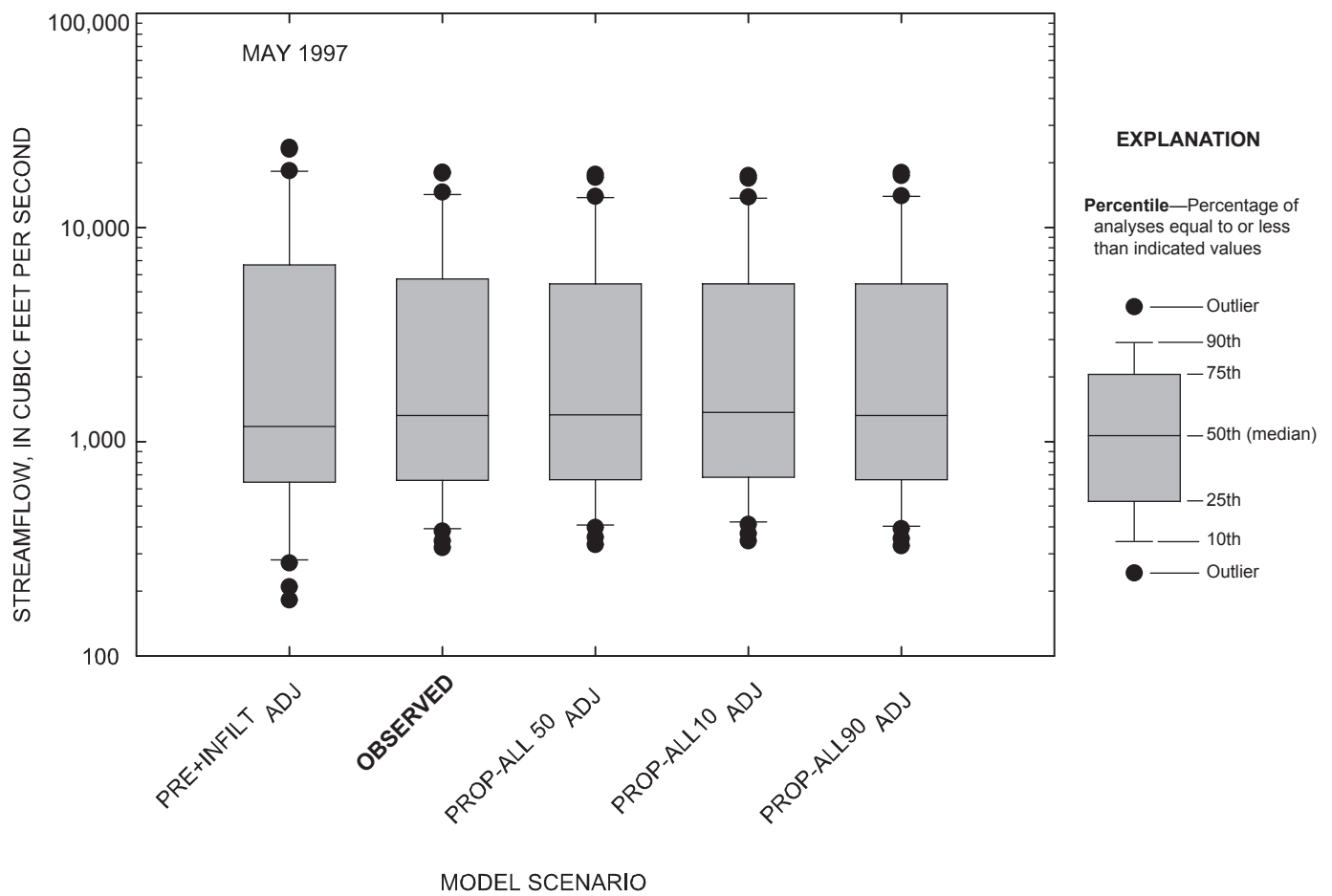
Figure 4-32. Comparison of daily streamflow for observed and simulated conditions at the Marais des Cygnes River near the Kansas-Missouri state line, Kansas, May 1997.
